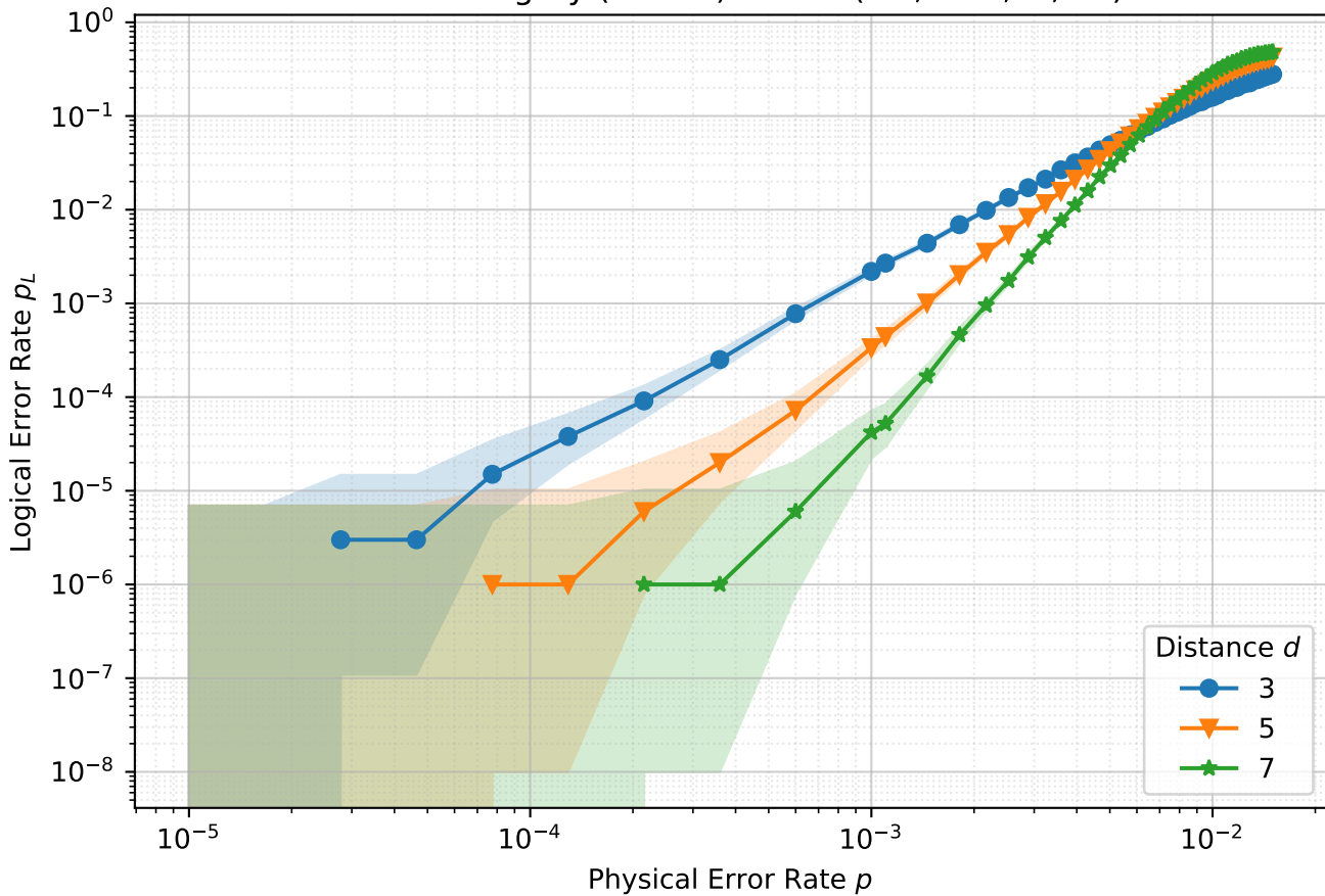
Lattice Surgery (Circuit)-Noise: ('I0', 'X+', 'I', 'X')
