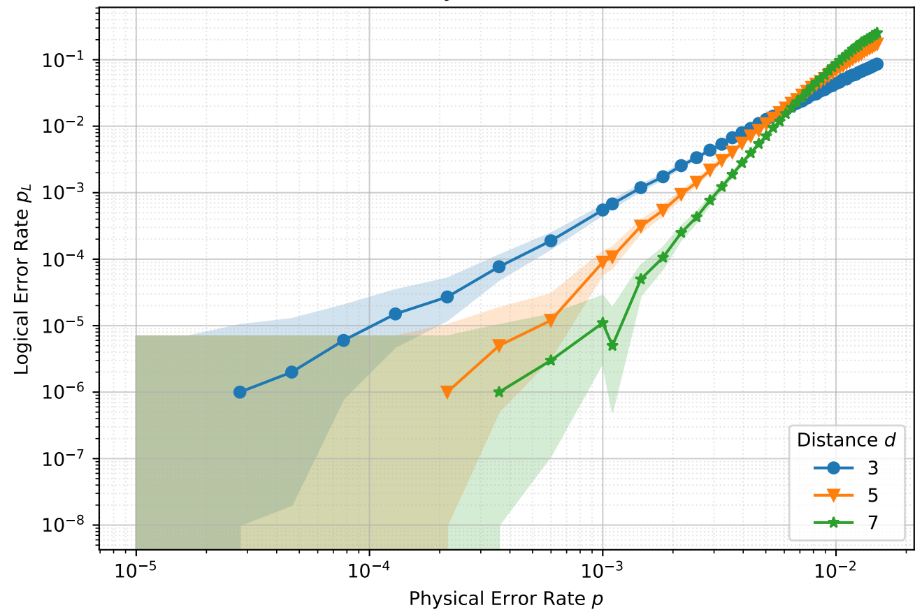
Surface Memory (Circuit)-Noise: ('Y+', 'Y')
