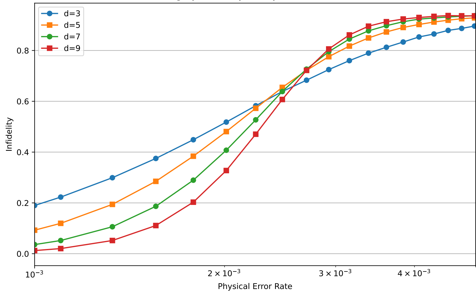
Surgery: Infidelity vs Physical Error Rate
