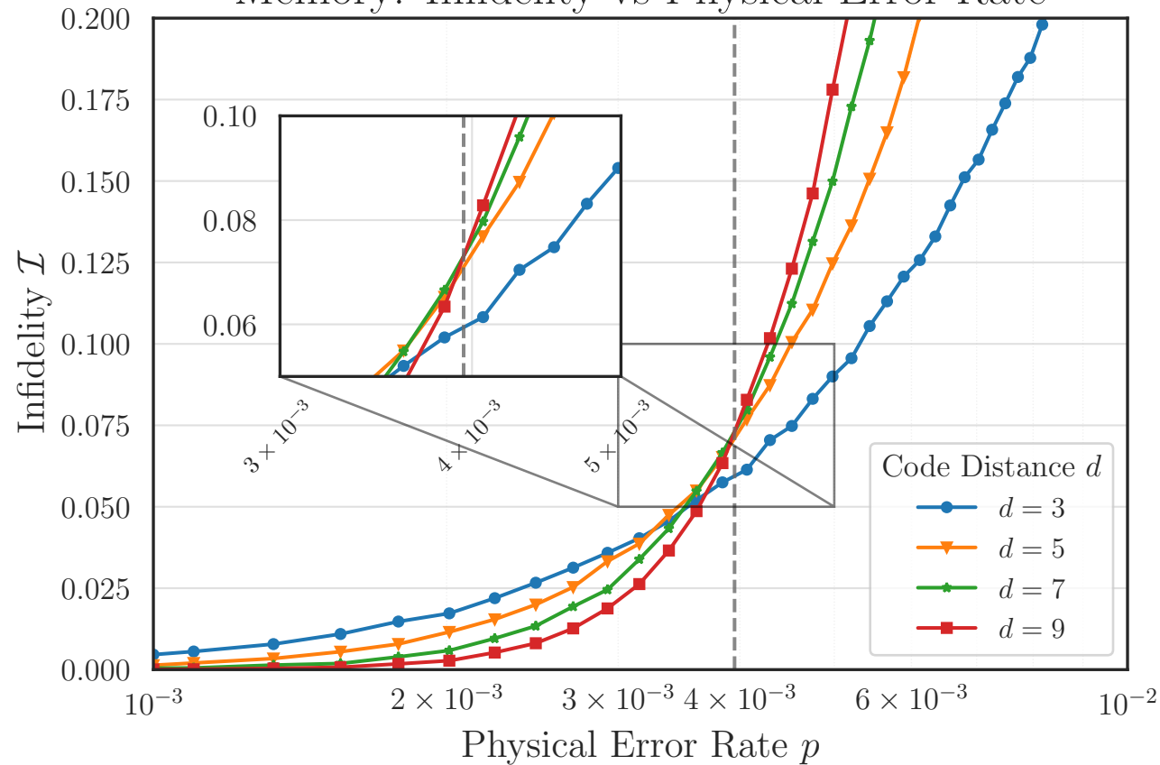
Memory: Infidelity vs Physical Error Rate
