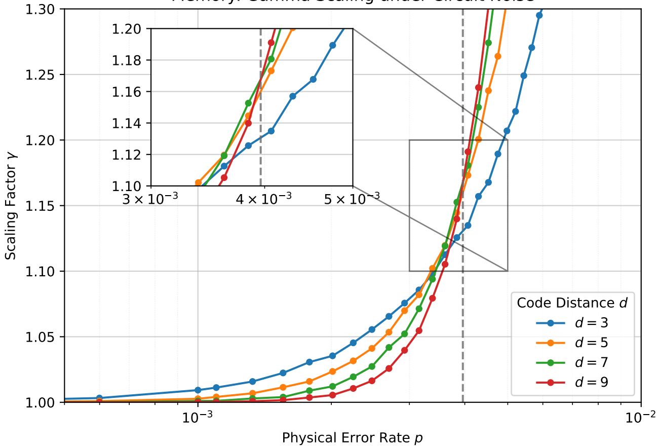
Memory: Gamma Scaling under Circuit Noise
