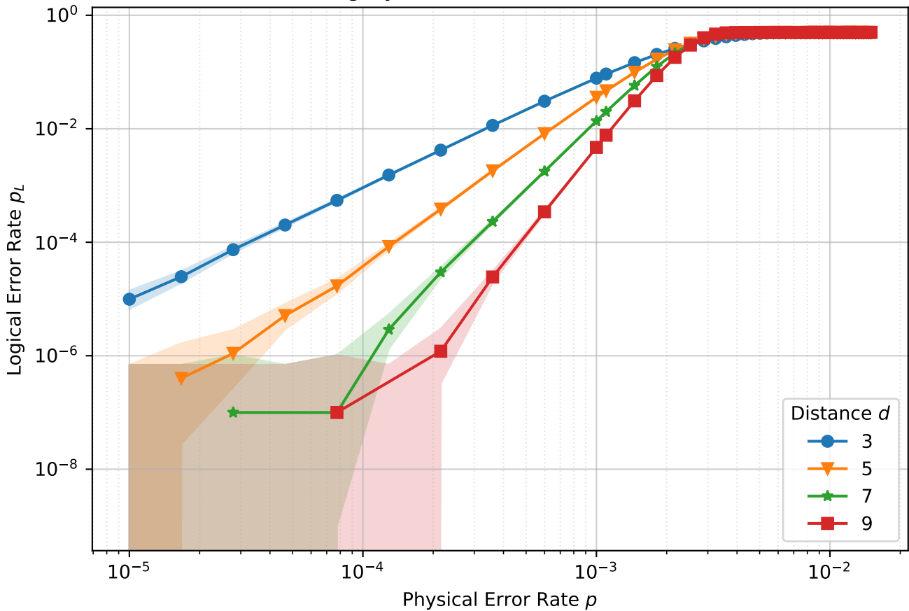
Lattice Surgery (Circuit)-Noise: ('X+', 'I0', 'X', 'X')
