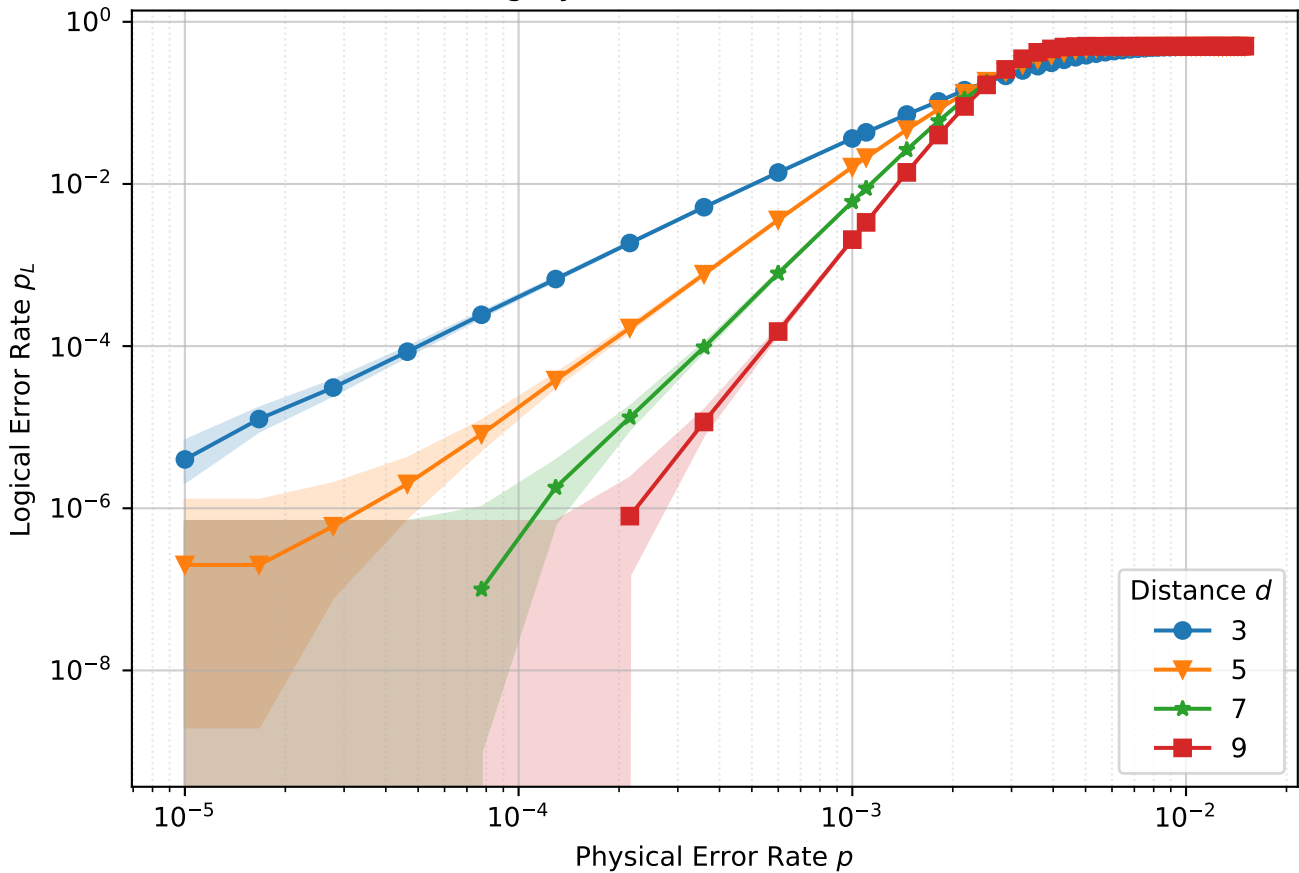
Lattice Surgery (Circuit)-Noise: ('Z0', 'I0', 'Z', 'I')
