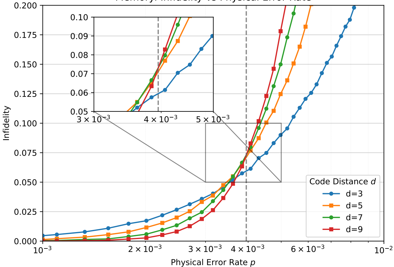
Memory: Infidelity vs Physical Error Rate
