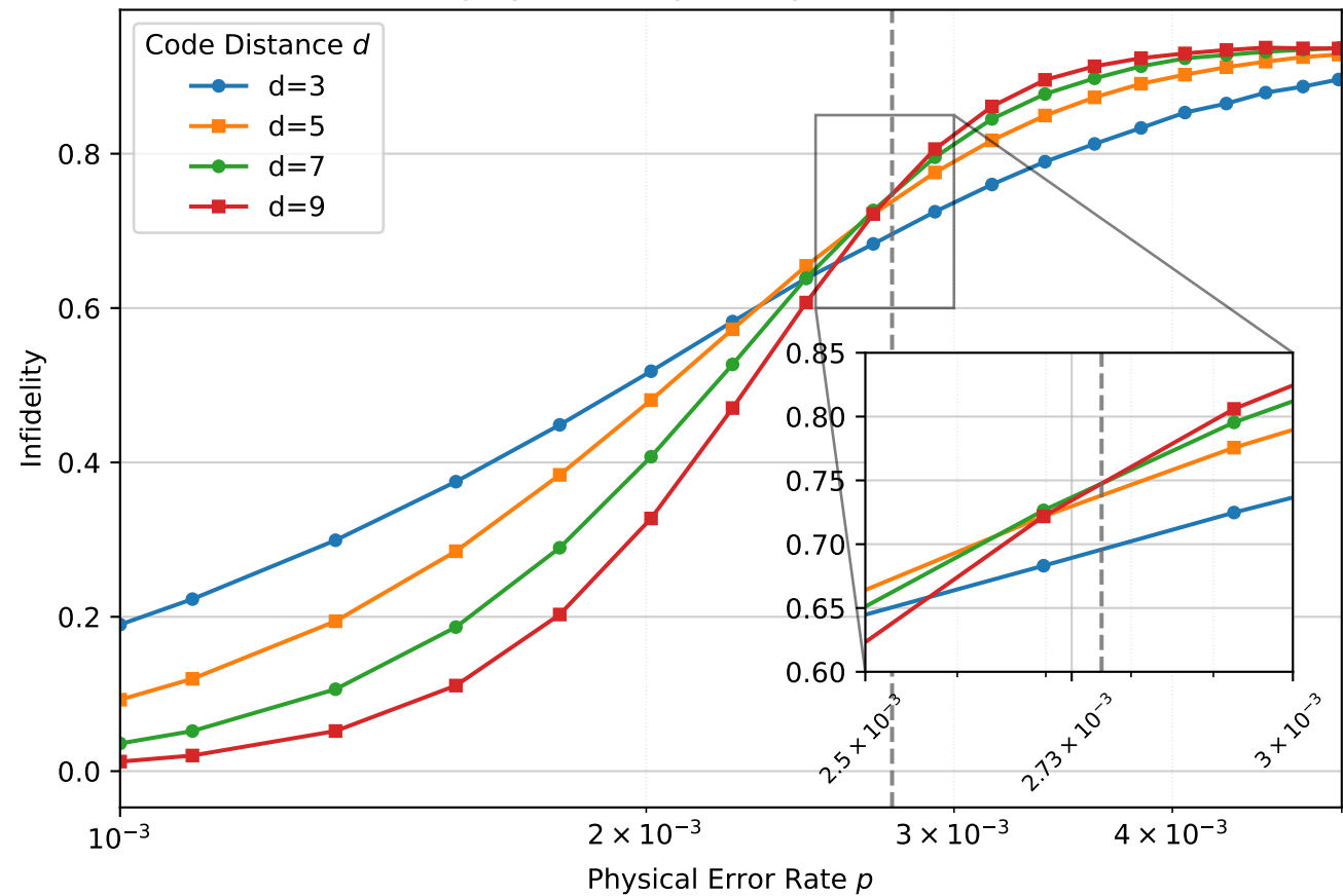
Surgery: Infidelity vs Physical Error Rate
