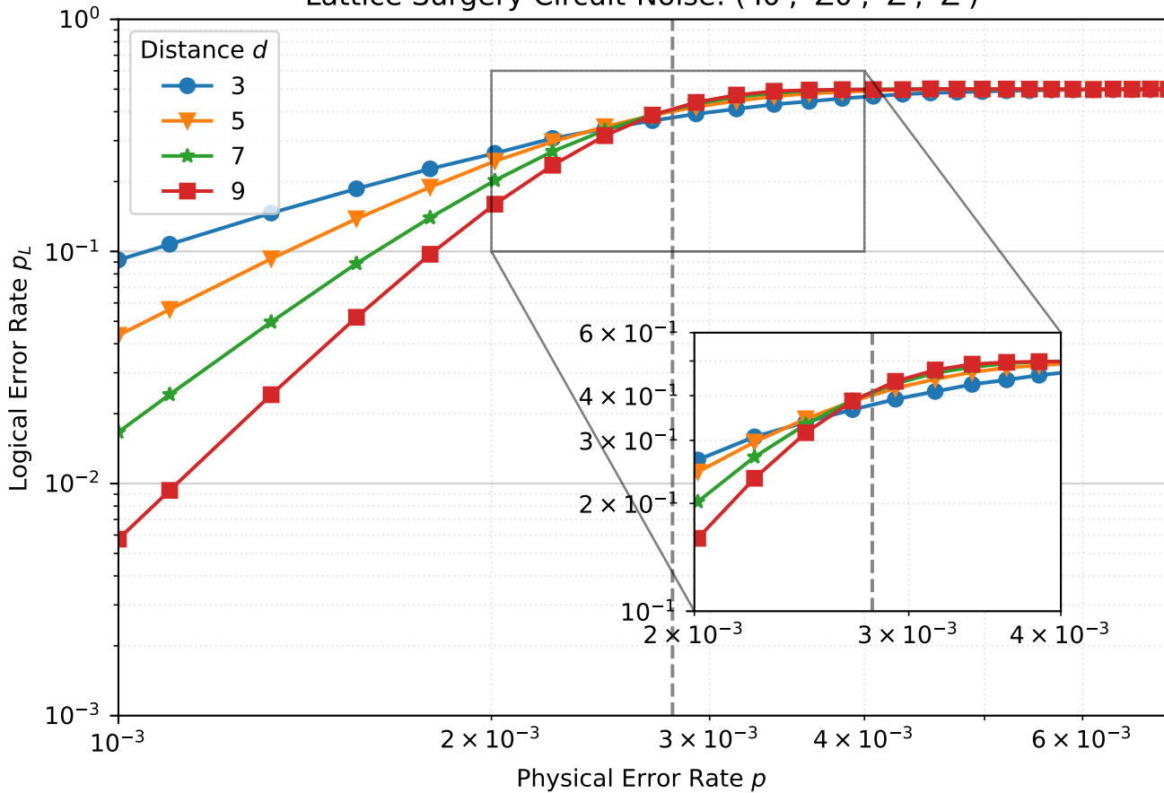
Lattice Surgery Circuit-Noise: ('I0', 'Z0', 'Z', 'Z')
