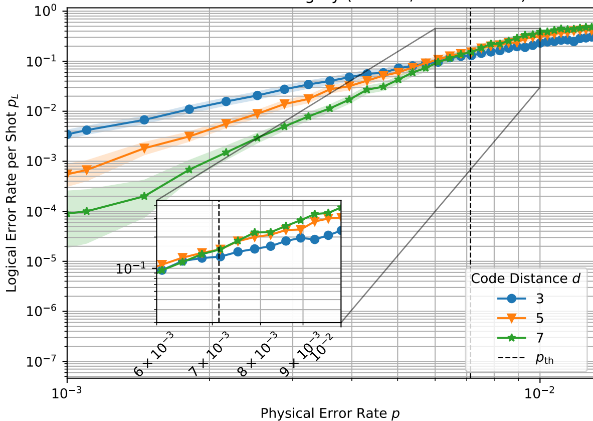
Threshold Lattice Surgery (XI→XX, Circuit Noise)
