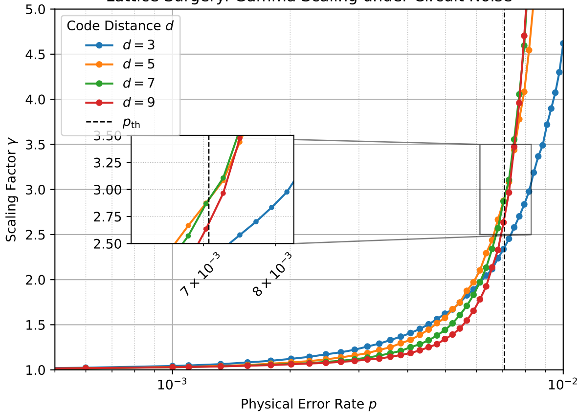
Lattice Surgery: Gamma Scaling under Circuit Noise
