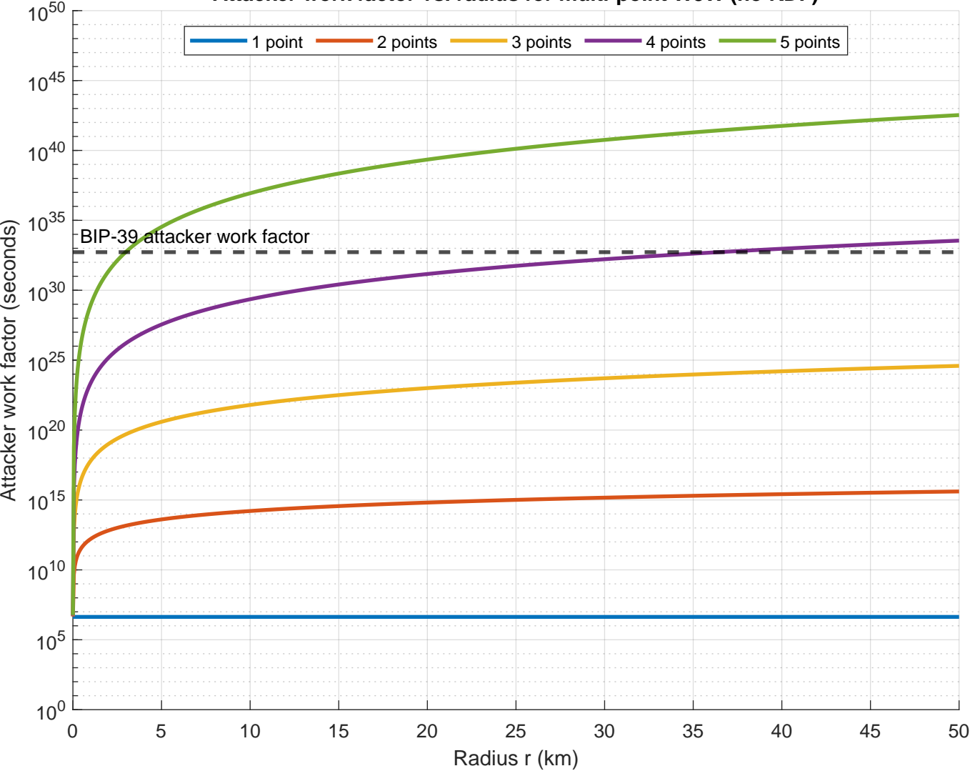
Attacker work factor vs. radius for multi-point W3W (no KDF)
