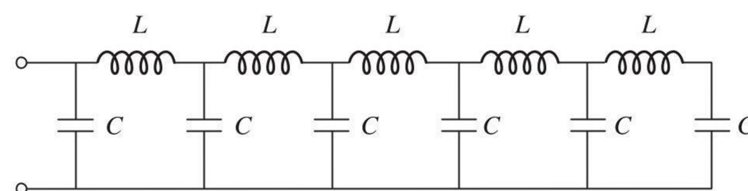
(c) Equivalent circuit
