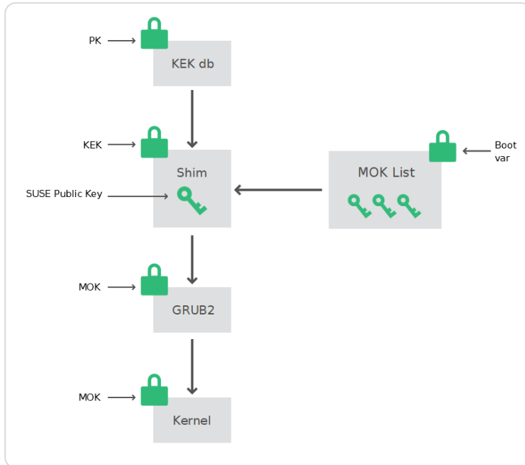
Figure 17.2. UEFI: secure boot process
