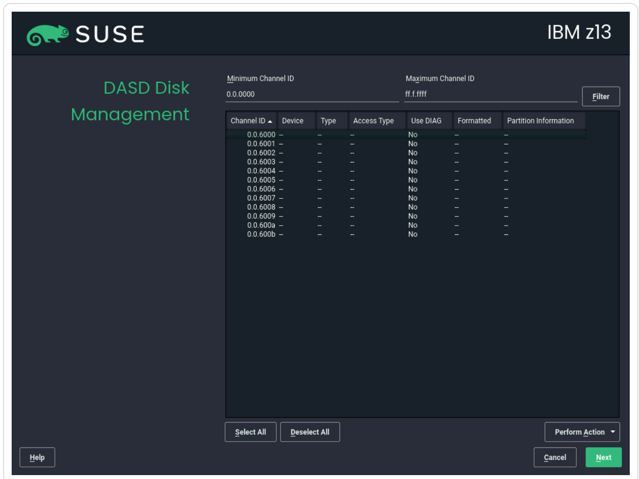
Figure 10.4. DASD disk management
