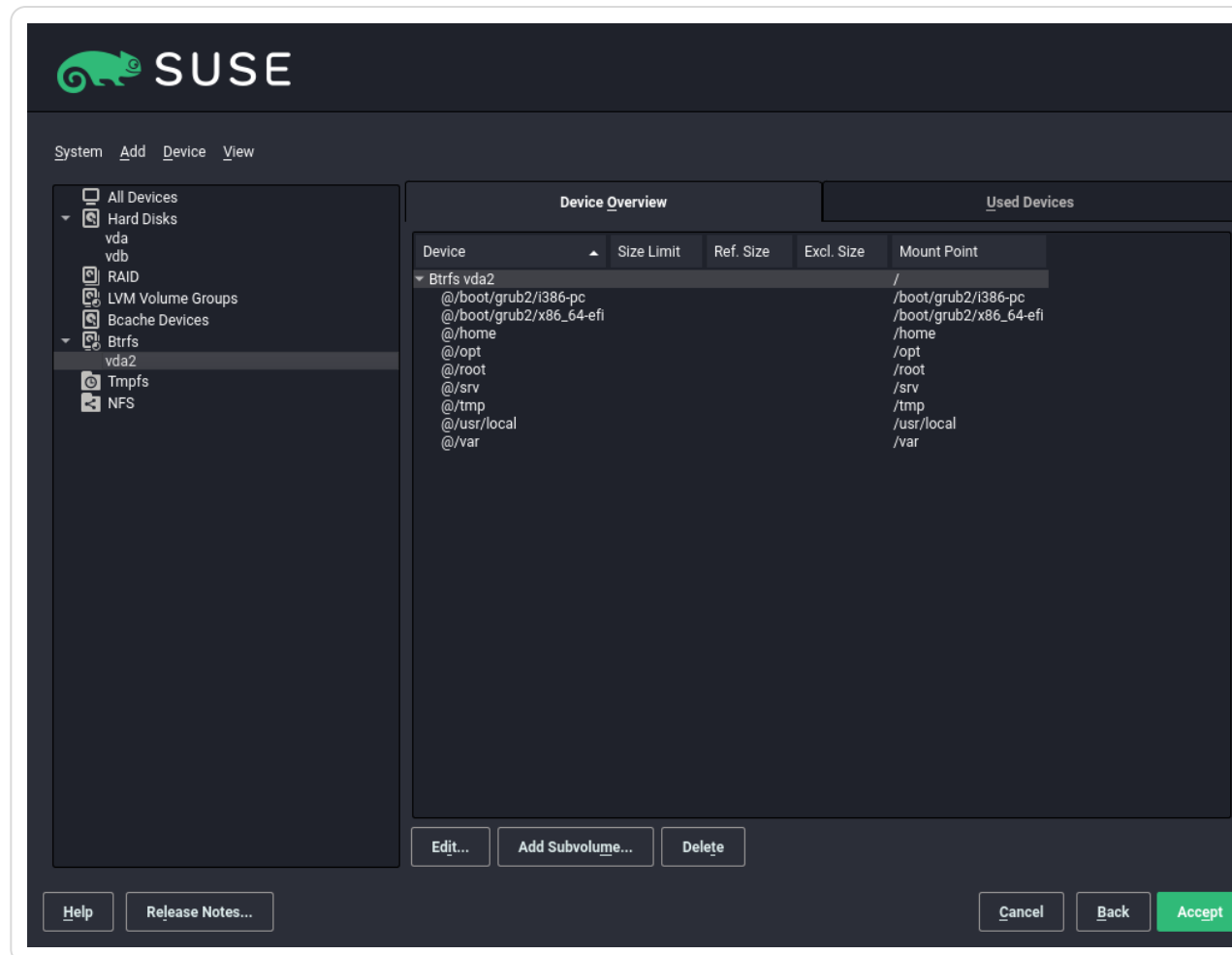
Figure 12.2. Btrfs subvolumes in YaST partitioner
