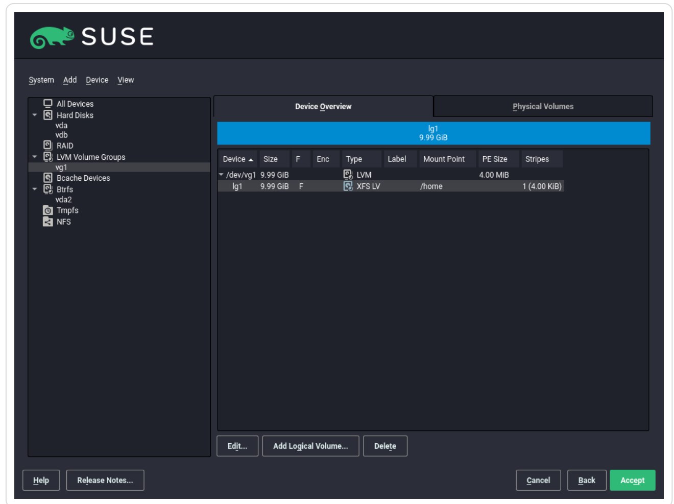
Figure 12.4. Logical volume management
