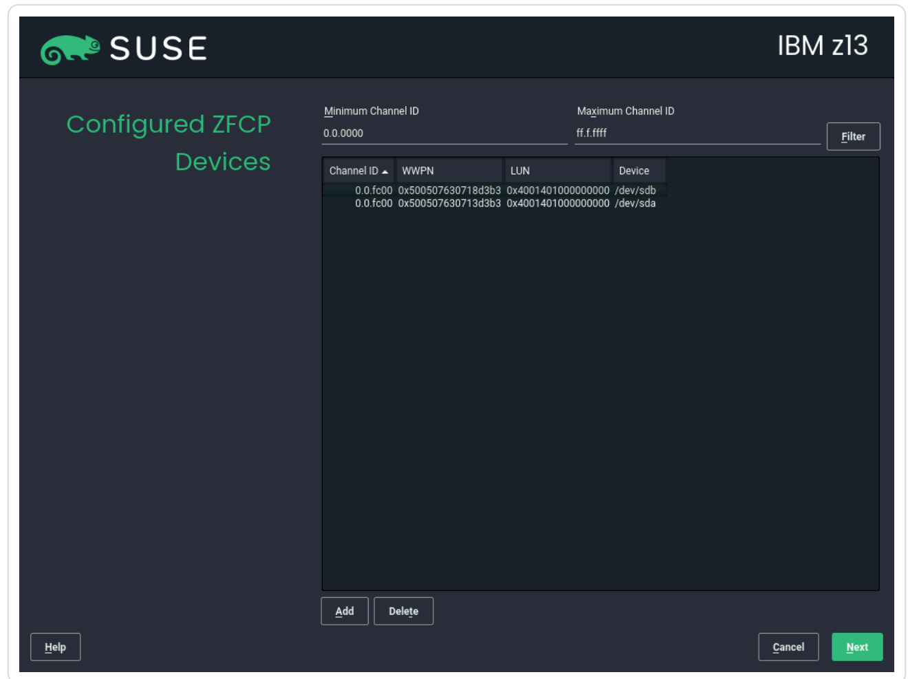
Figure 10.5. Configured zFCP Devices
