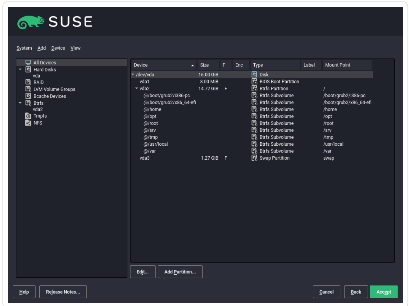
Figure 12.1. The YaST partitioner
