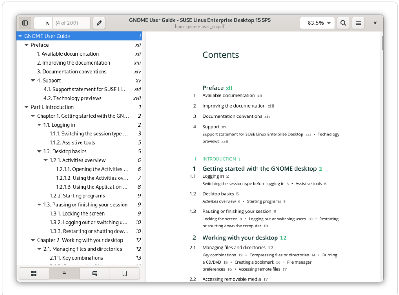
Figure 2.3. Document viewer
