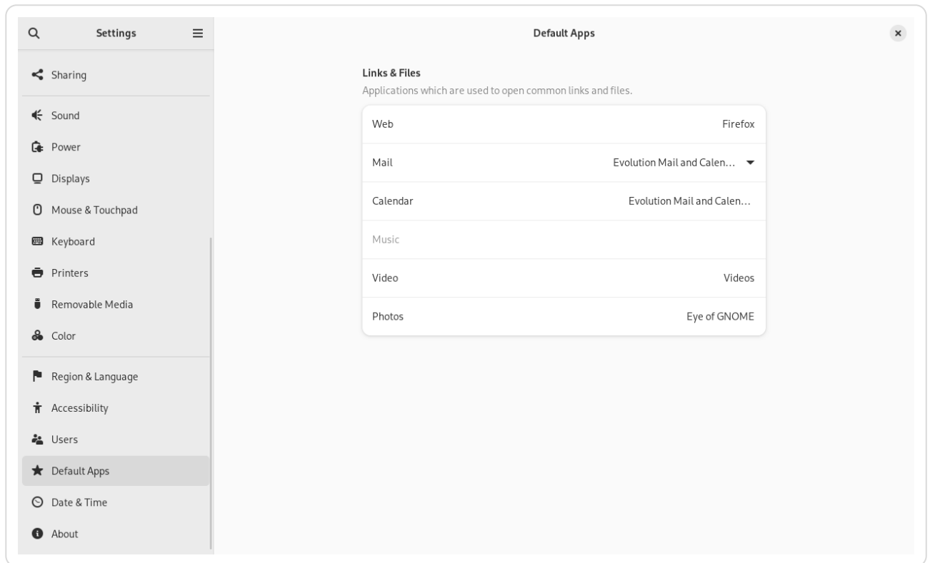
Figure 3.6. Default Apps
