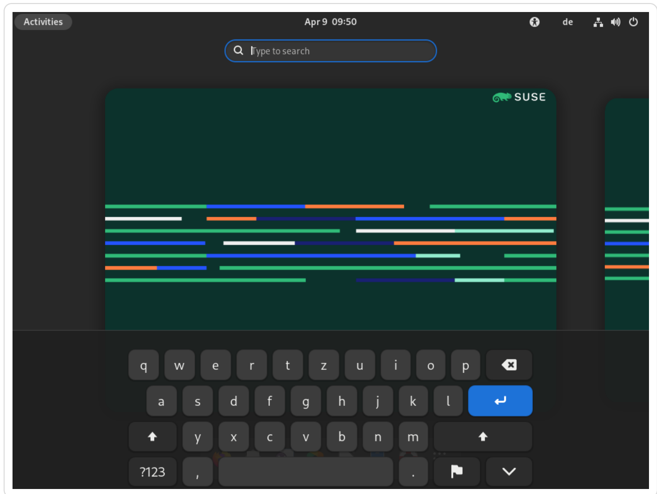
Figure 4.1. On-screen keyboard
