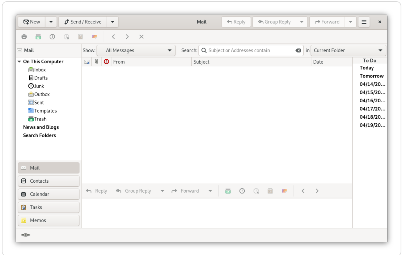
Figure 14.1. Evolution window
