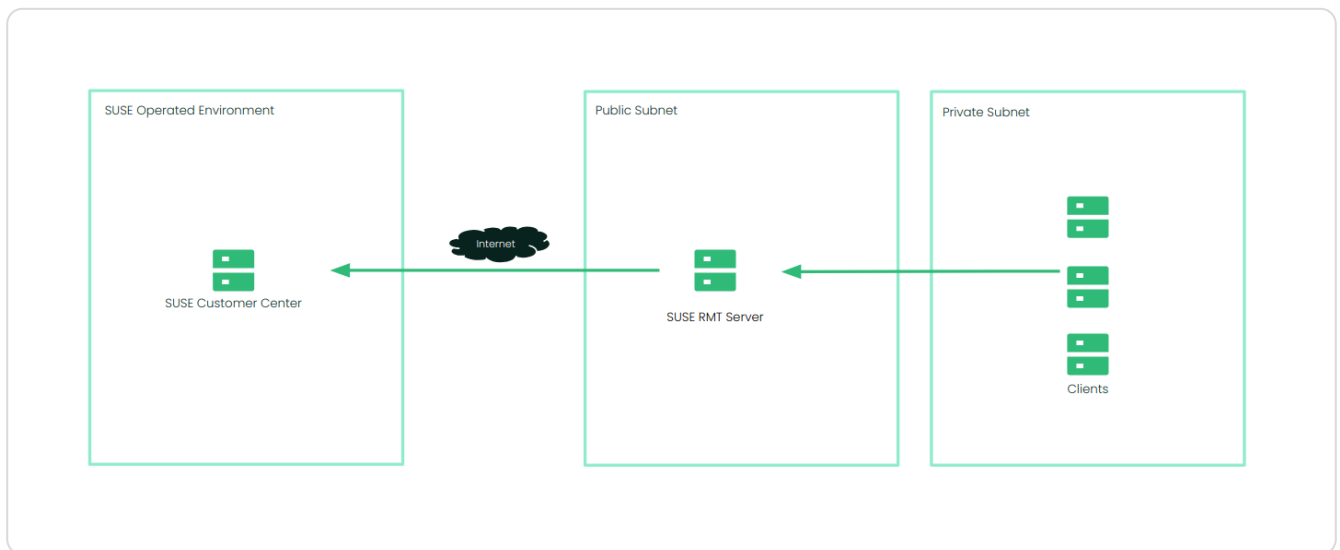
Figure 9.1. An example of cloud architecture for RMT deployment
