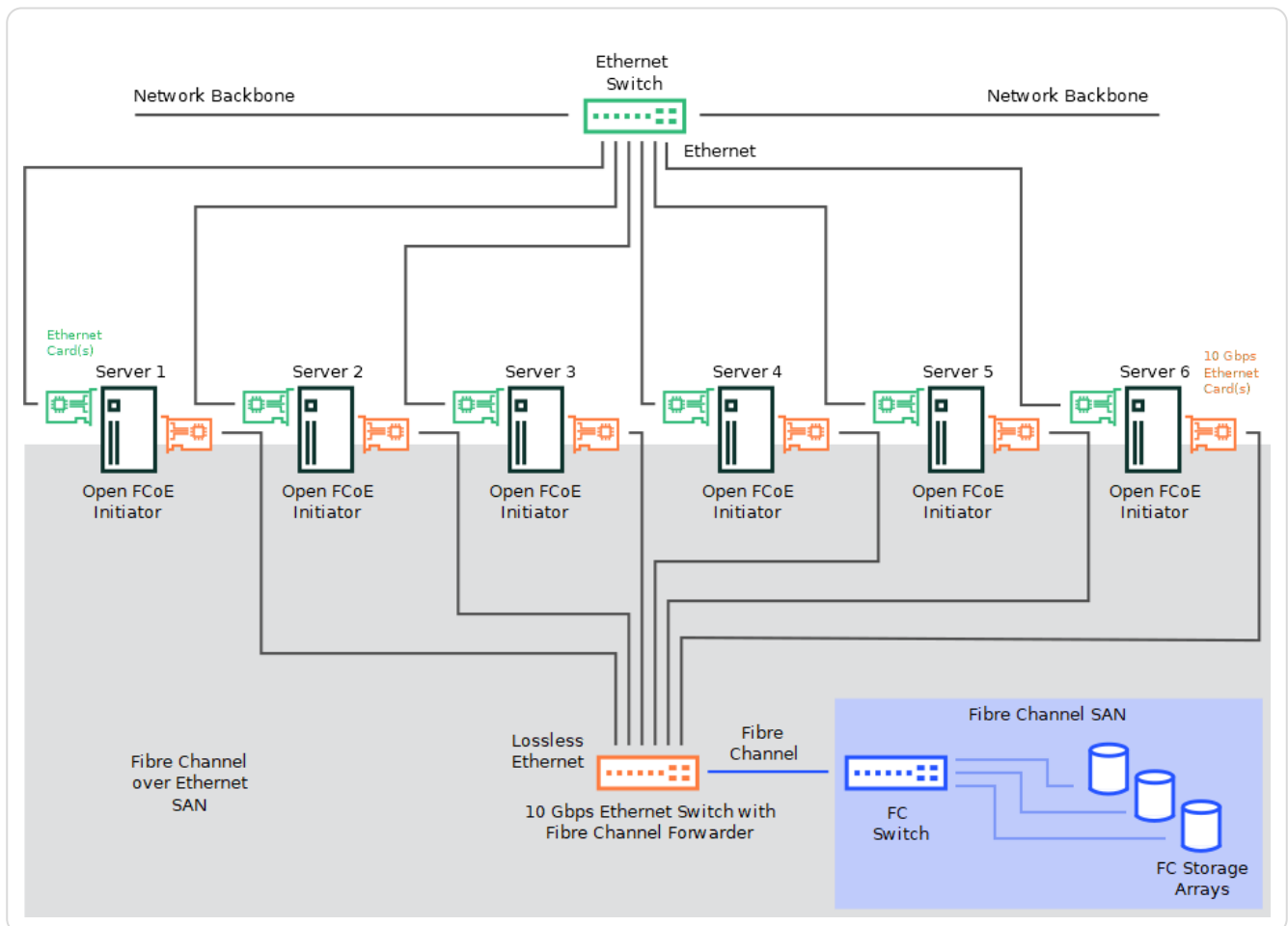
Figure 16.1. Open Fibre channel over Ethernet SAN
