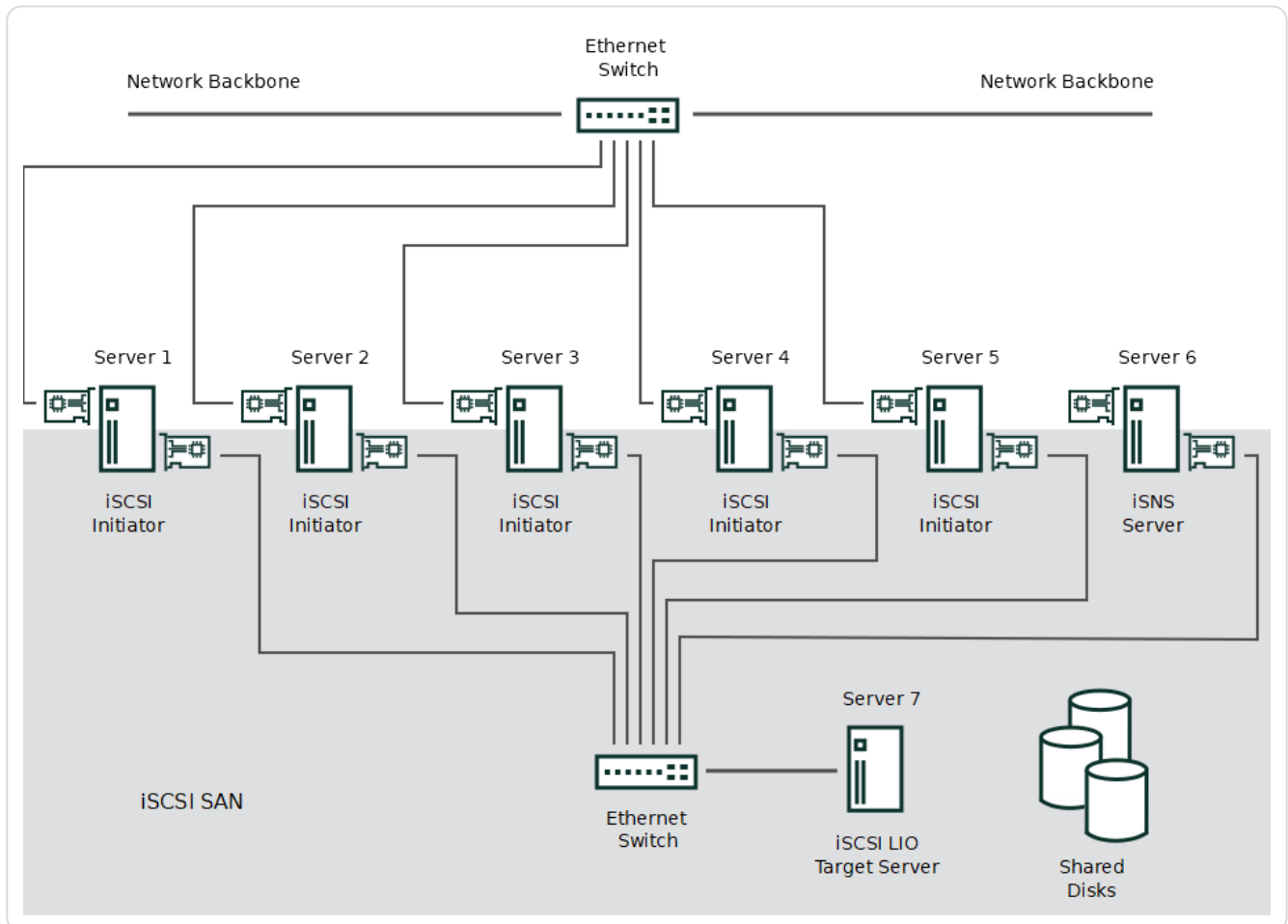
Figure 15.1. iSCSI SAN with an iSNS server
