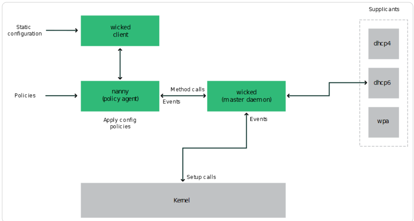
Figure 23.6.1.1.4. wicked architecture
