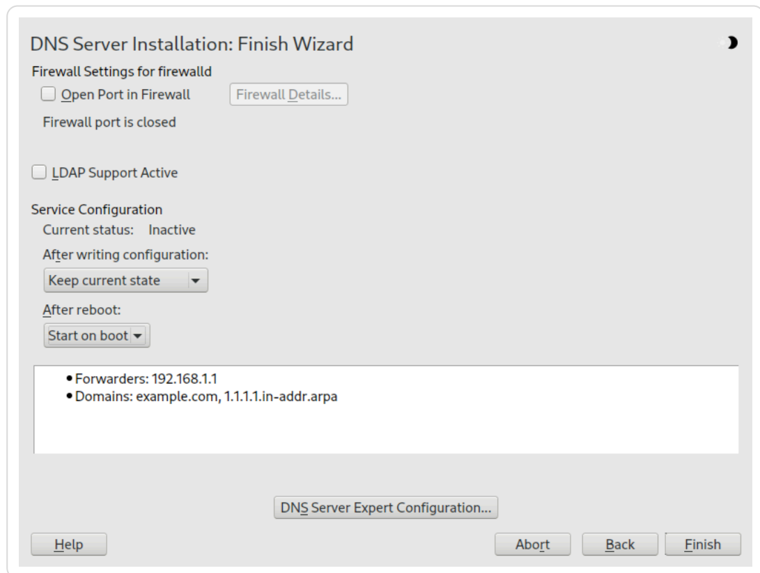
Figure 40.3.1.3. DNS server installation: finish wizard
