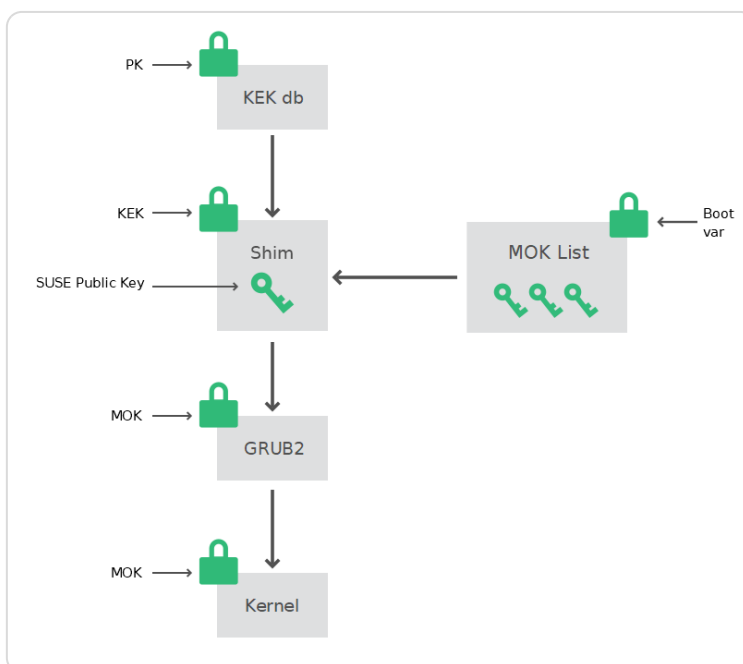
Figure 17.1.1.2. UEFI: secure boot process
