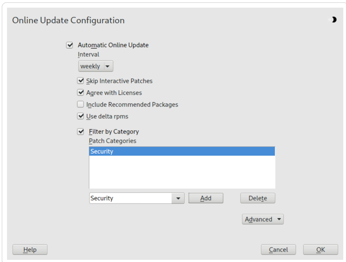
Figure 7.4.3. YaST online update configuration
