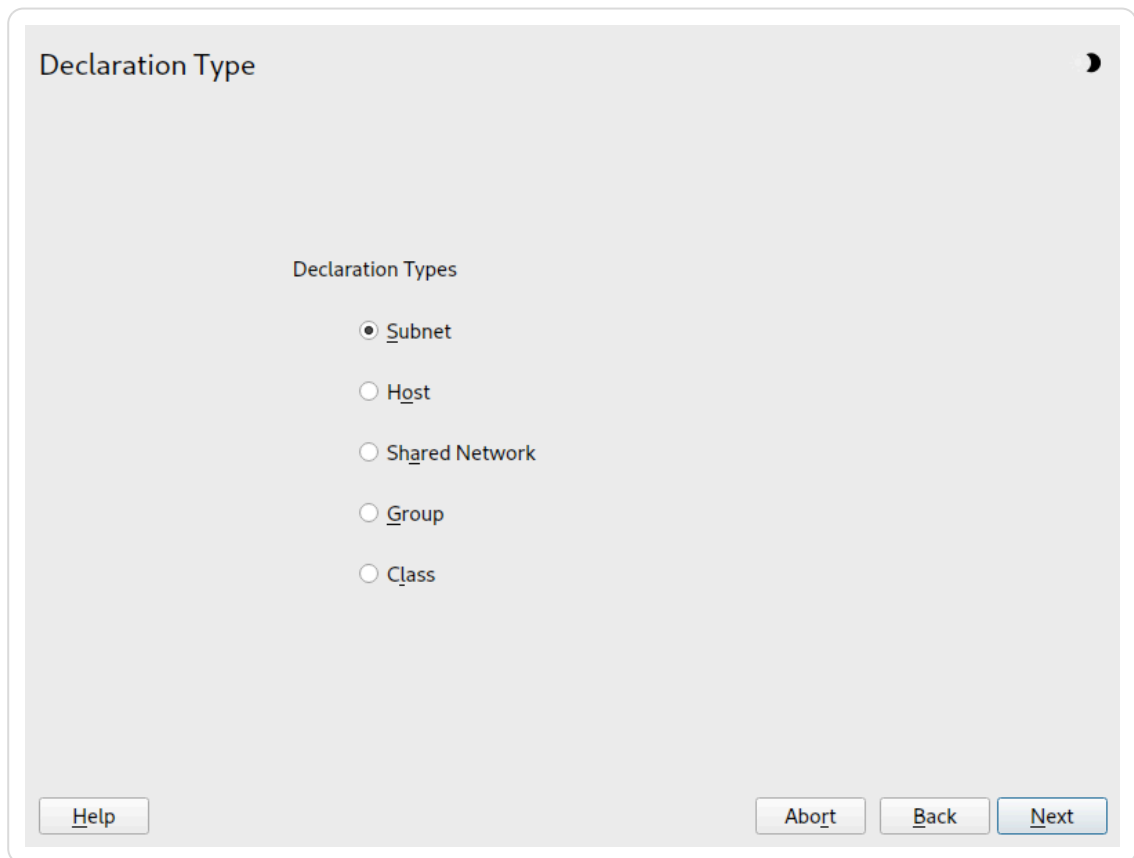
Figure 41.1.2.7. DHCP server: selecting a declaration type
