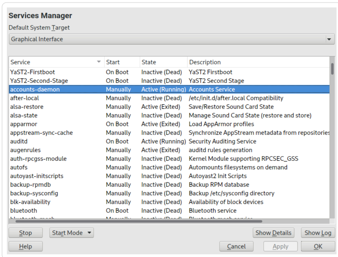
Figure 19.4.1. Services Manager
