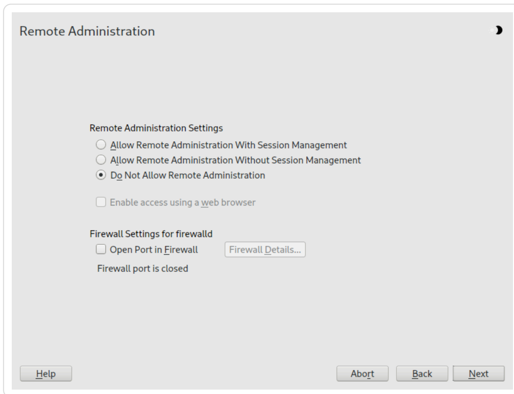
Figure 14.3.7. Remote administration
