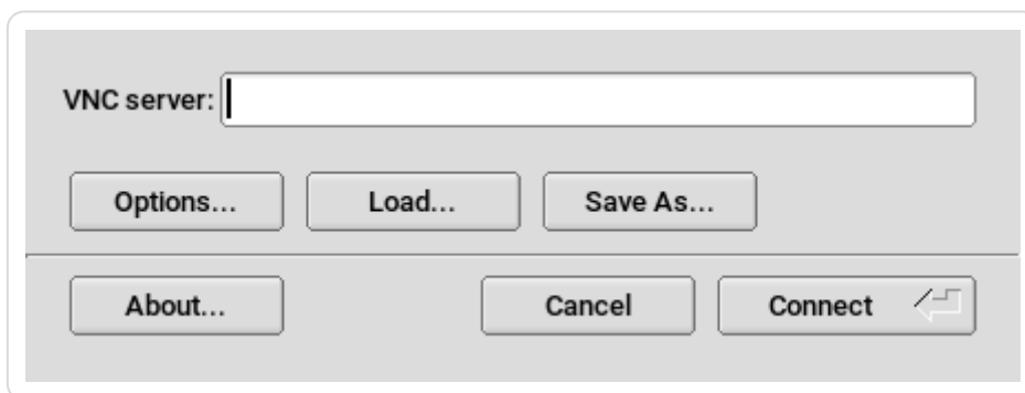
Figure 14.1.2.1. vncviewer
