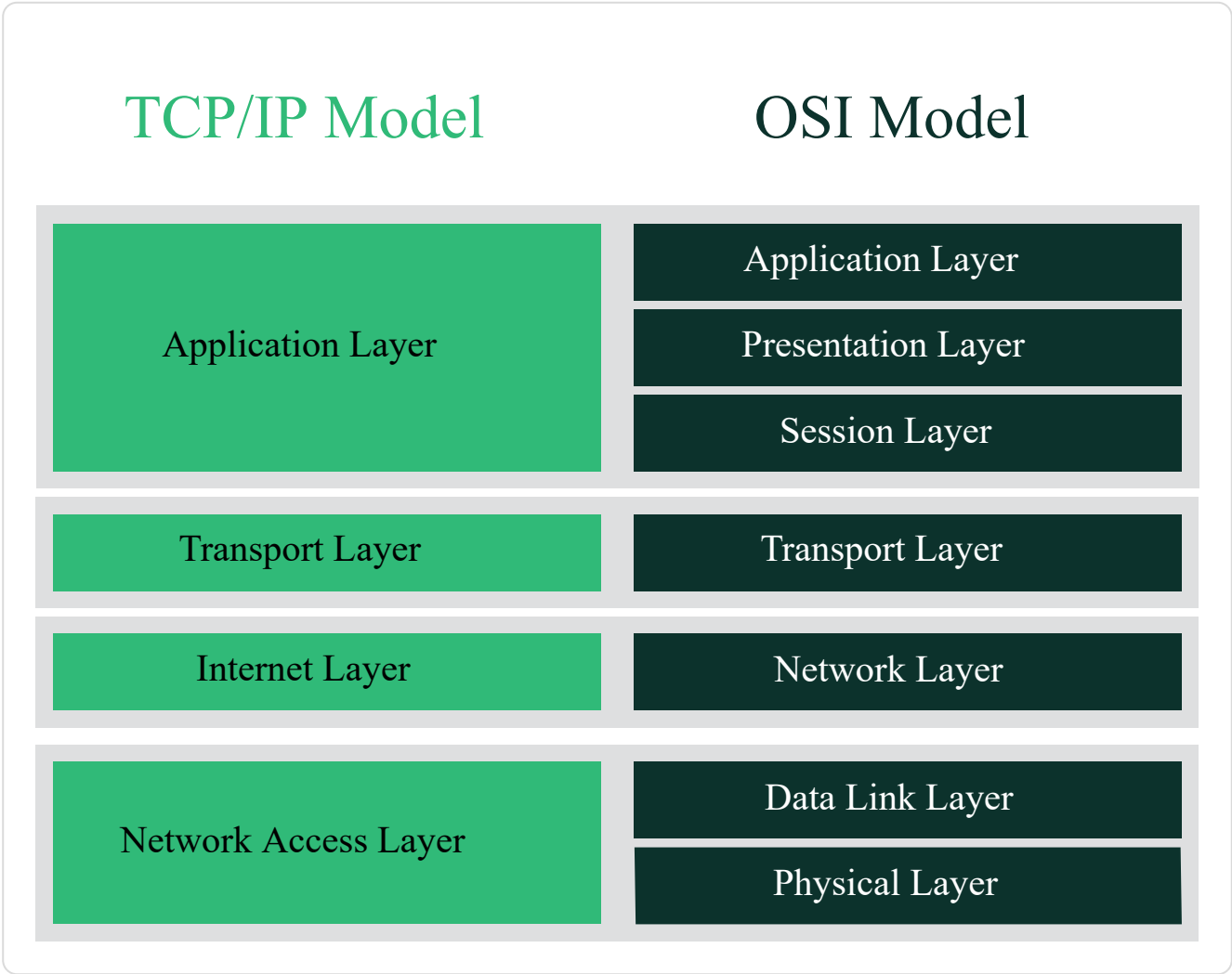
Figure 23.1. Simplified layer model for TCP/IP
