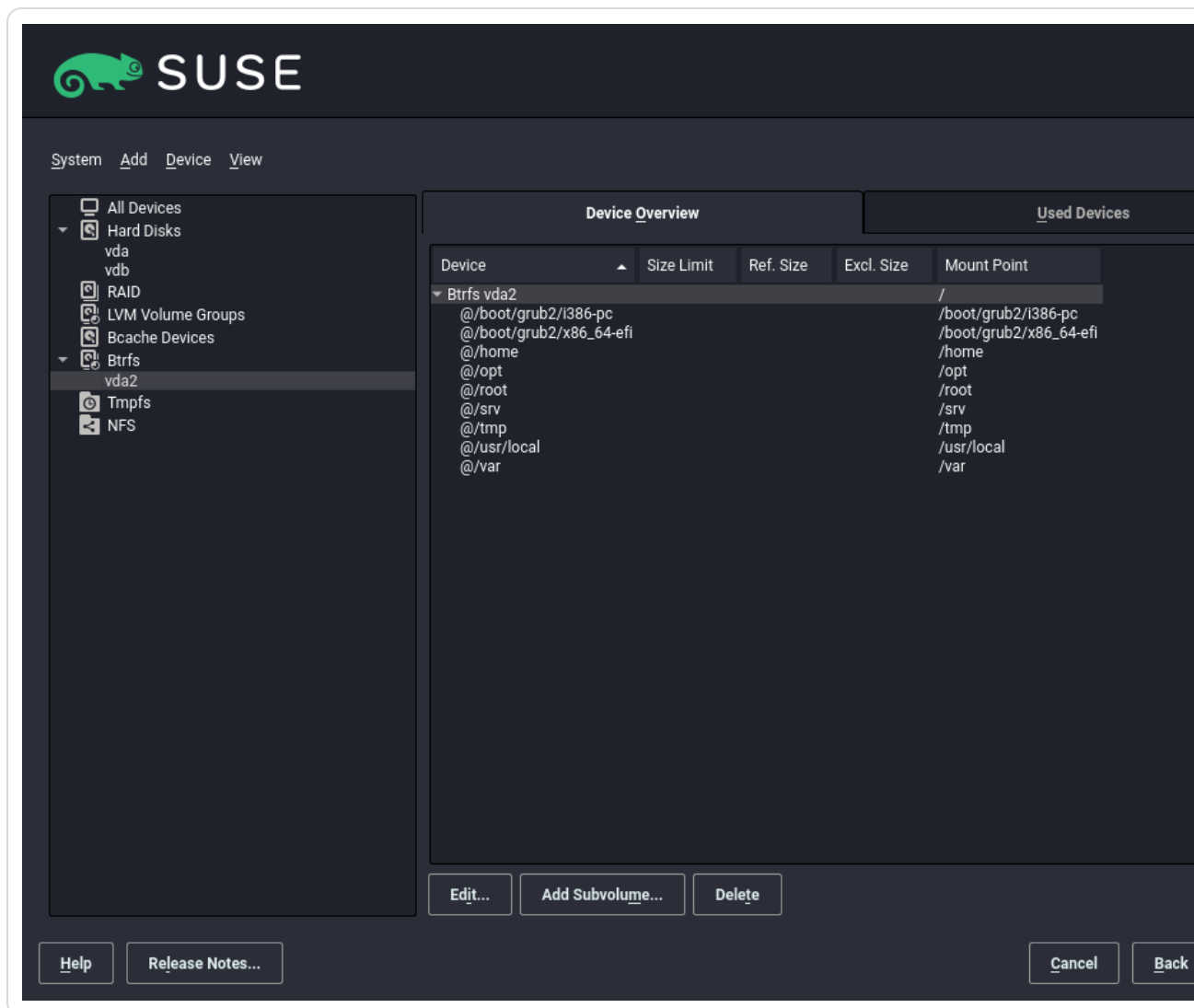
d. Figure 12.1.2.3.2. Btrfs subvolumes in YaST partitioner
