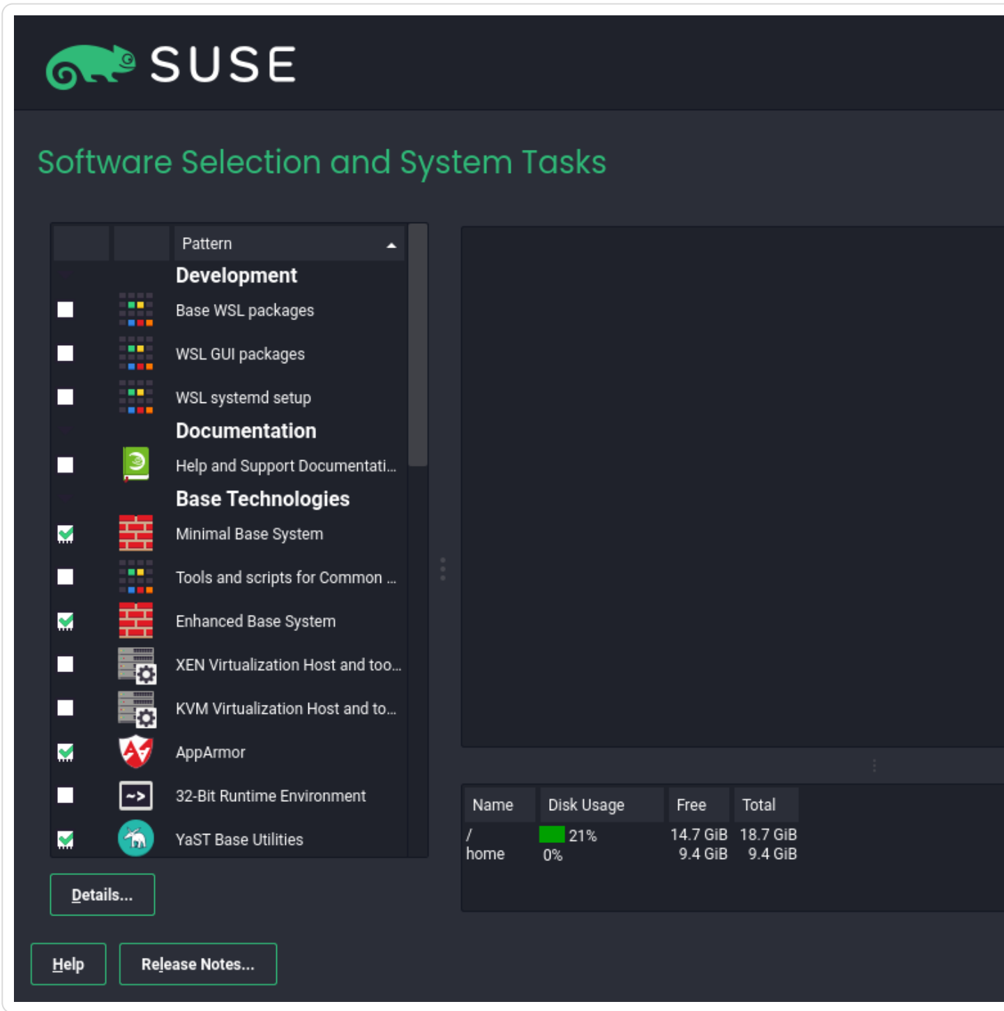
Figure 10.15.1.16. Software selection and system tasks
