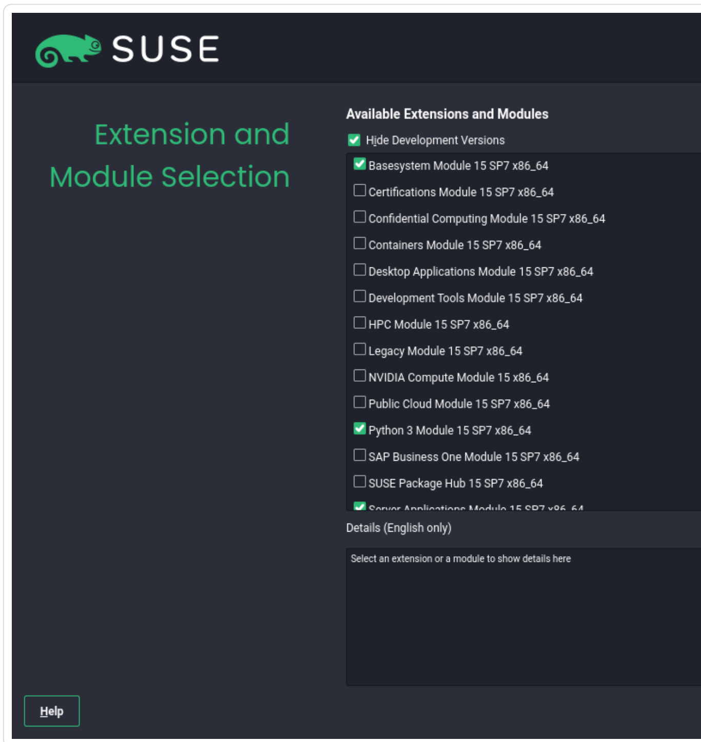
Figure 10.8.8. Extension and module selection
