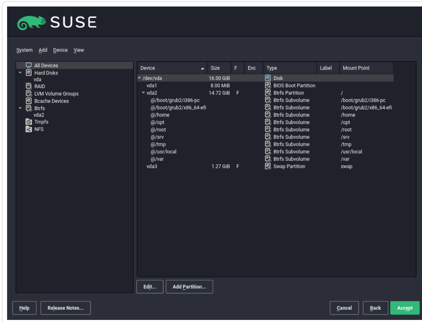
Figure 12.1.1. The YaST partitioner
