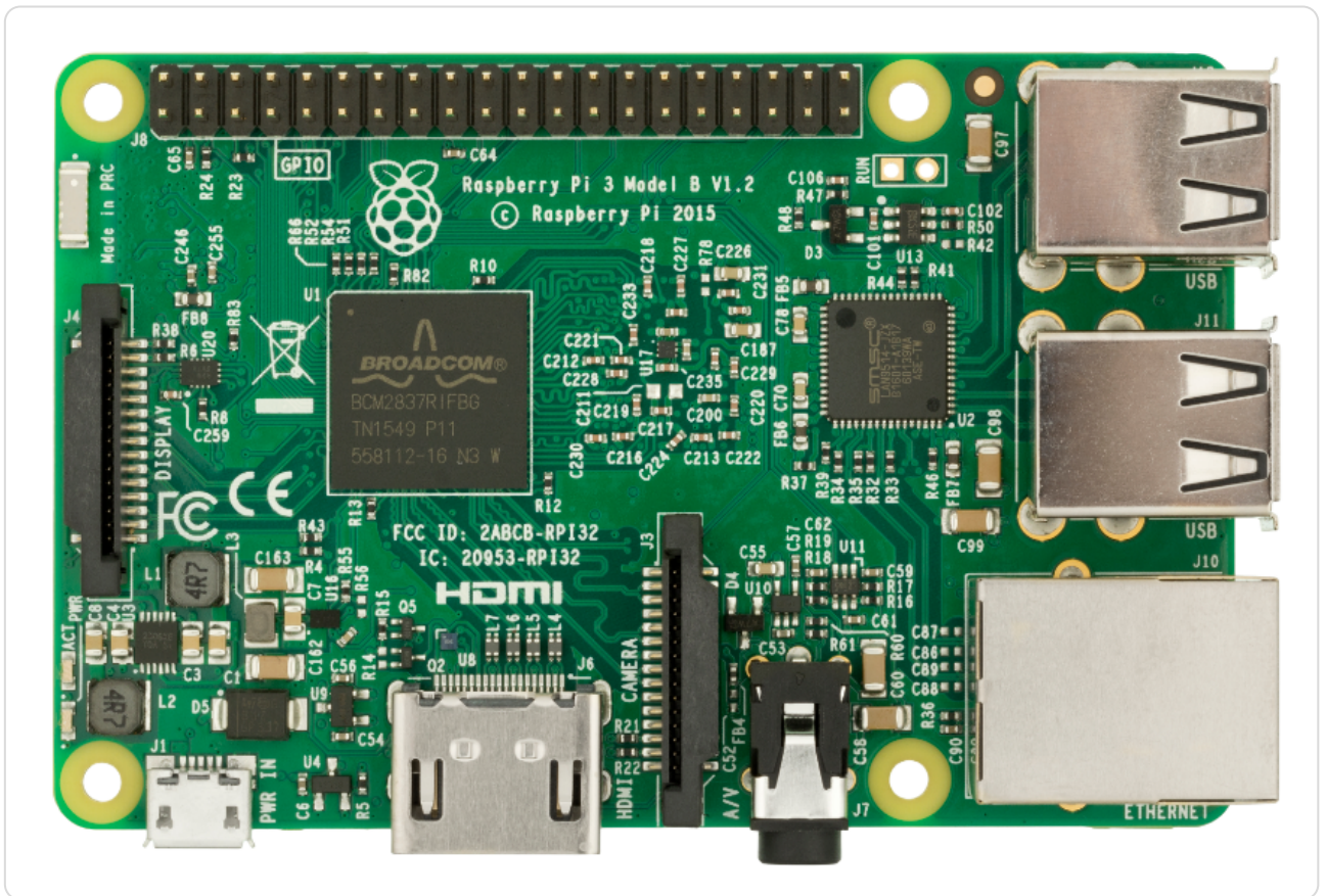
Figure 1.1.2. Photo of Raspberry Pi 3 model B connectors, © Evan-Amos / own work / public domain
