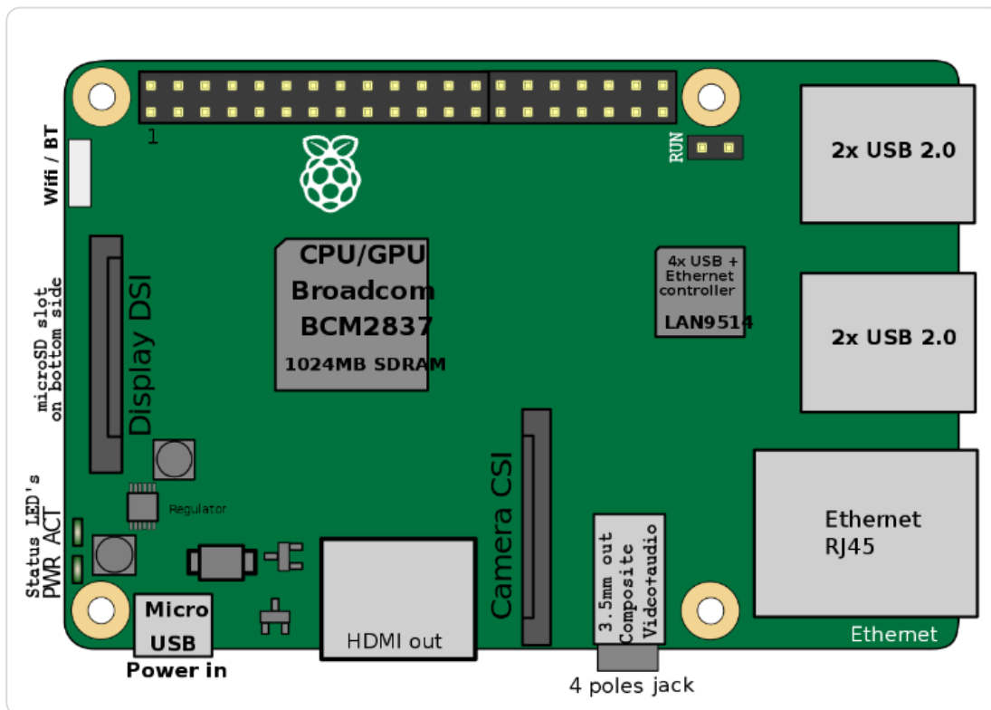
Figure 1.1.1. Overview of Raspberry Pi 3 model B connectors, © Efa / English Wikipedia / CC BY-SA 3.0
