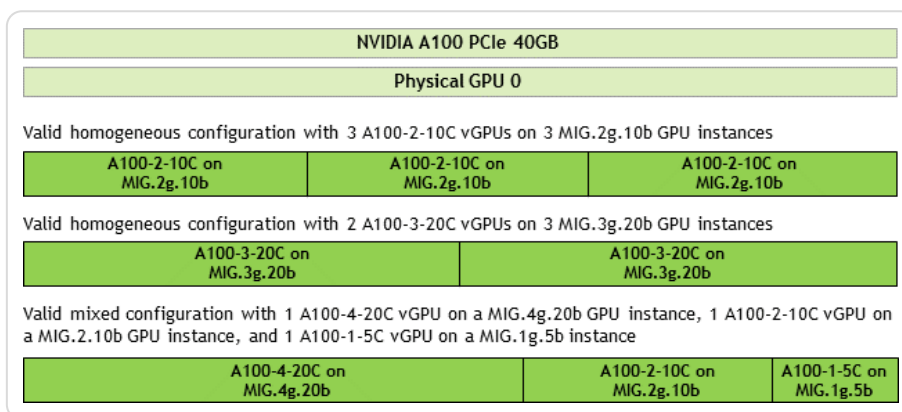
Figure 11.3.2.4. Example MIG-backed vGPU configurations on NVIDIA A100 PCIe 40 GB PCIe 40 GB (source: https://docs.nvidia.com/grid/latest/grid-vgpu-user-guide/index.html )
