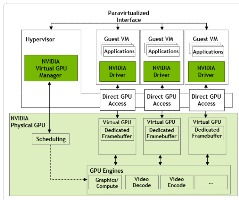
Figure 11.1.1. Time-sliced architecture (source: https://docs.nvidia.com/grid/latest/grid-vgpu-user-guide/index.html )
