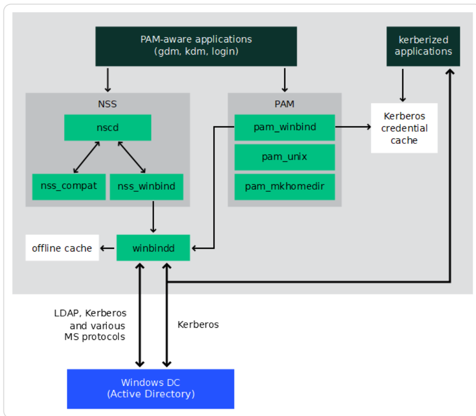
Figure 7.2.1. Schema of Winbind-based Active Directory authentication
