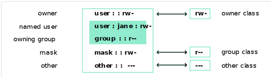
Figure 19.4.1.2. Extended ACL: ACL entries compared to permission bits
