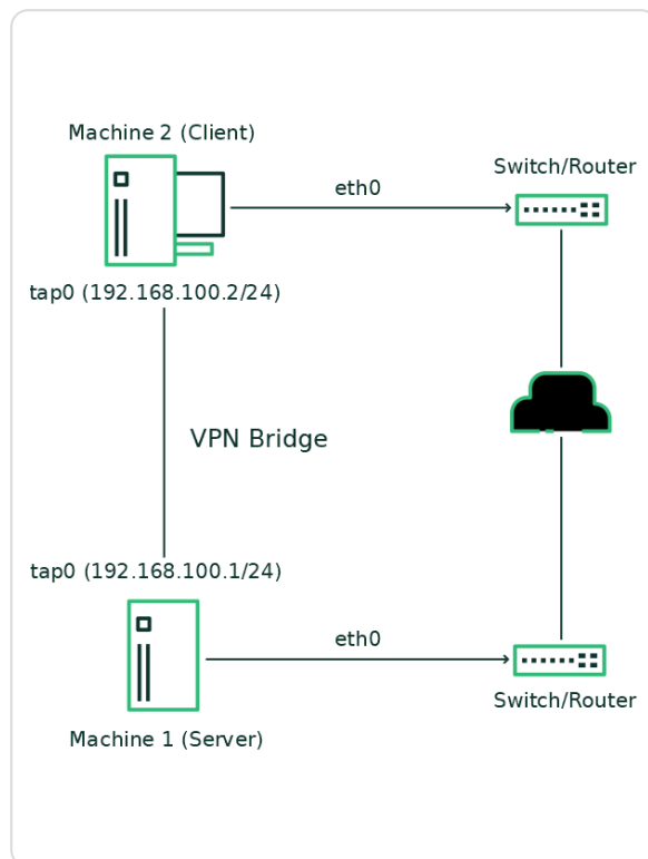
Figure 24.1.2.2. Bridged VPN - scenario 1
