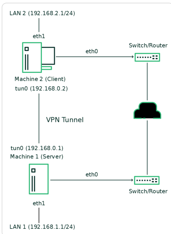
Figure 24.1.2.1. Routed VPN
