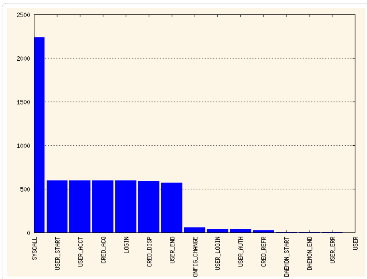
Figure 44.8.3. Bar chart—common event types
