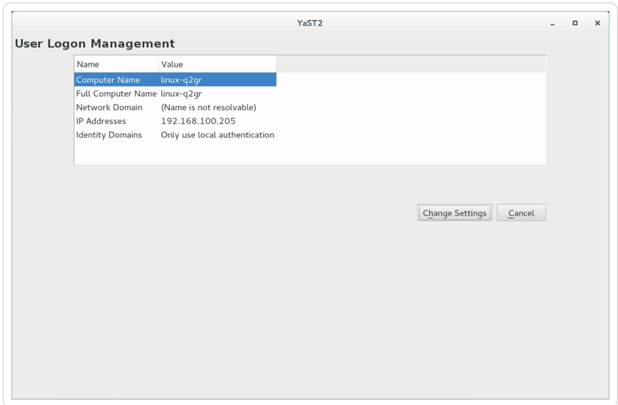
Figure 7.3.2.2. Main window of User logon management
