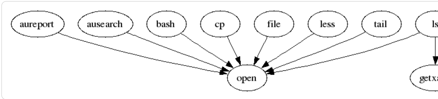
Figure 44.8.2. Flow graph—program versus system call relationship
