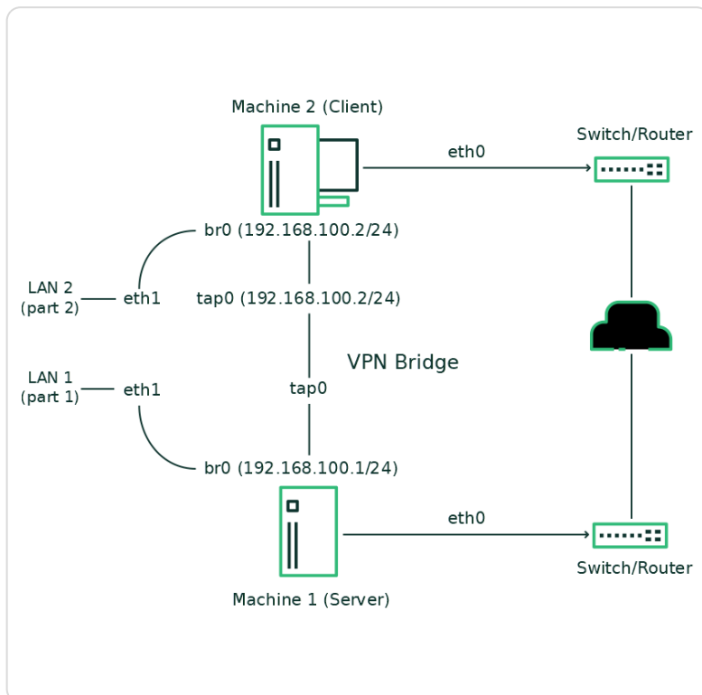
Figure 24.1.2.4. Bridged VPN - scenario 3
