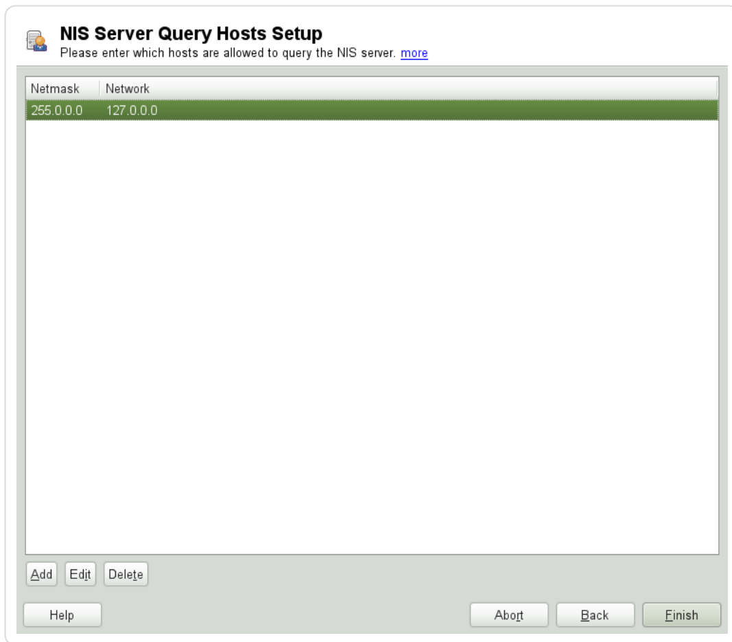
Figure 3.1.1.5. Setting request permissions for a NIS server
