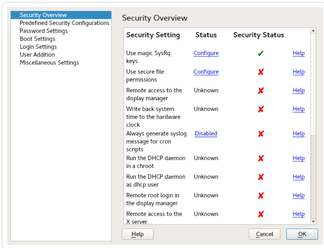
Figure 17.1.1. YaST security center and hardening: security overview
