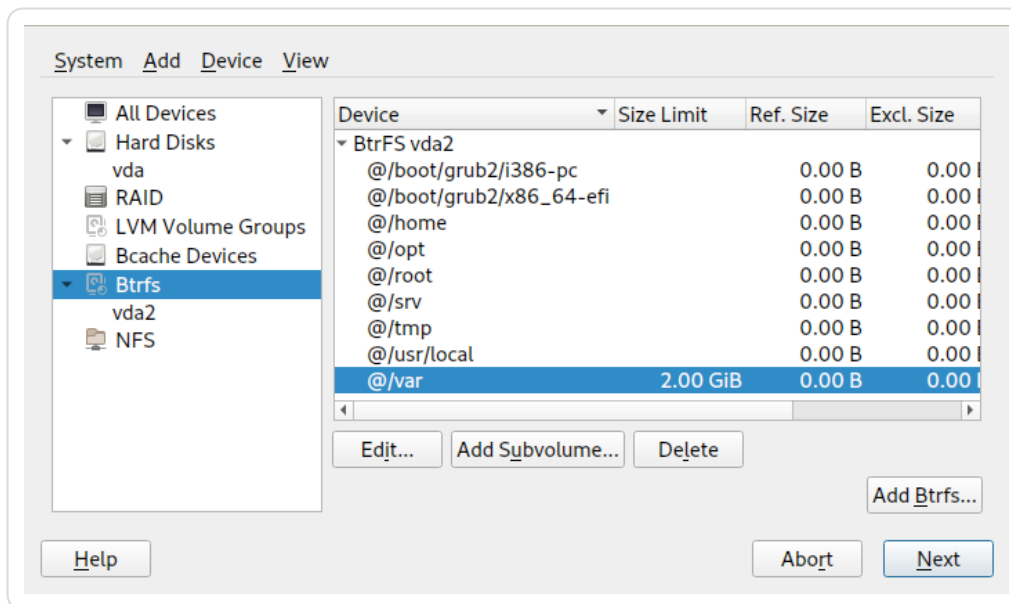
Figure 1.2.5.1.3. List of subvolumes for a device
