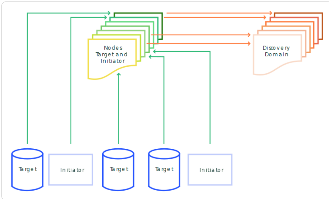
Figure 14.1.1. iSNS discovery domains
