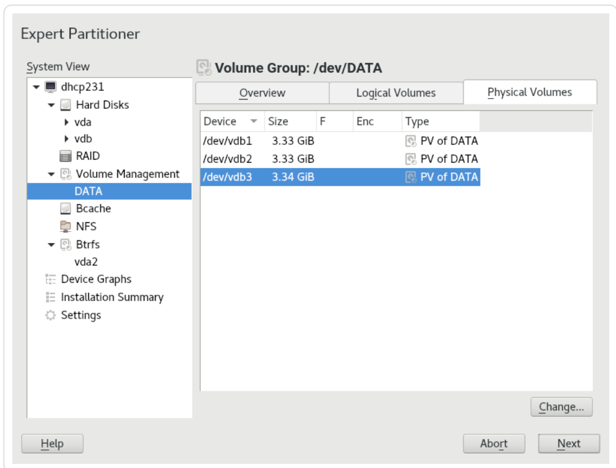
Figure 5.2.2. Physical volumes in the volume group named DATA
