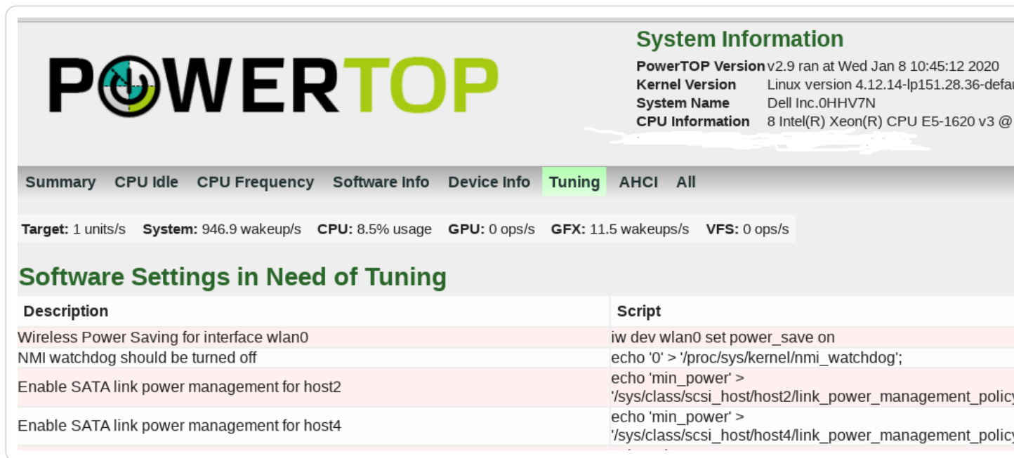
Figure 12.7.2. HTML powerTOP report
