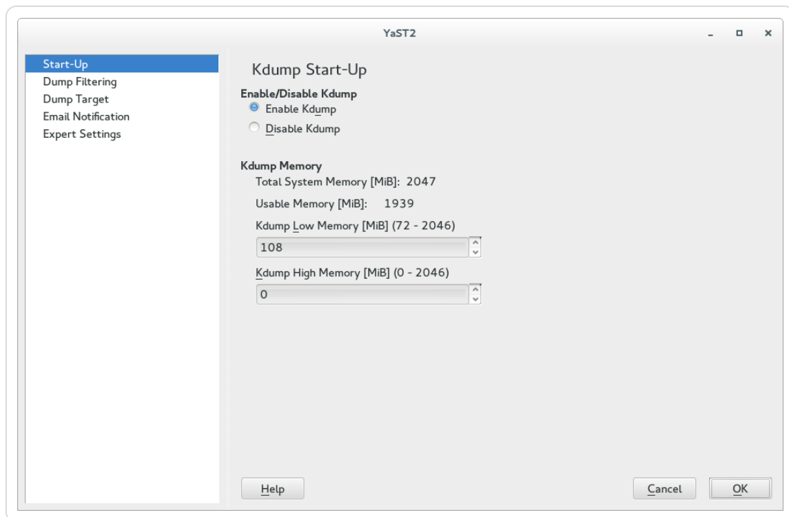
Figure 20.7.2.1. YaST Kdump module: start-up page
