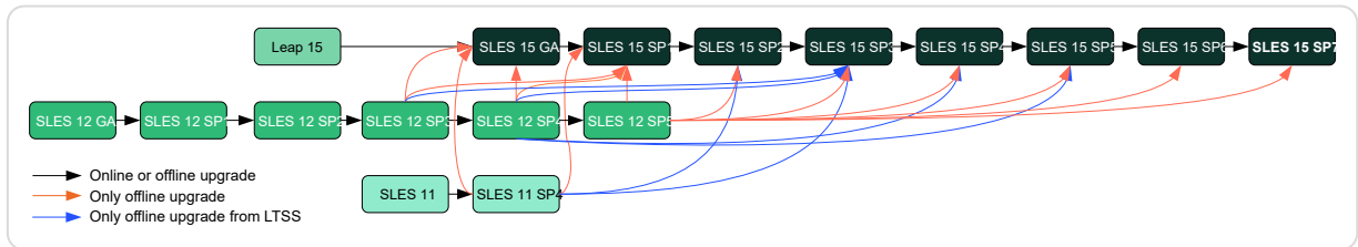
Figure 2.3.1. Overview of supported upgrade paths
