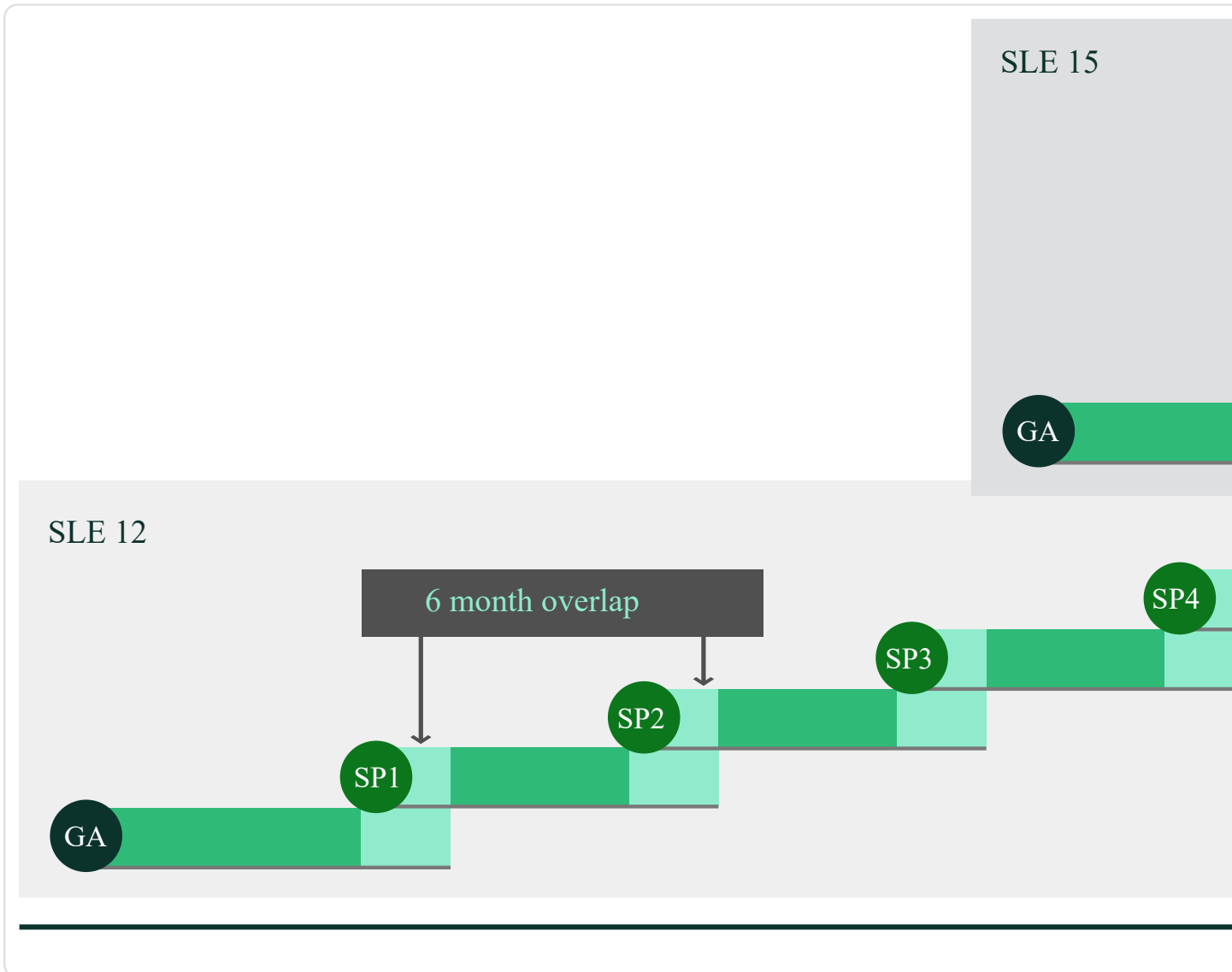
Figure 1.2.1. Major releases and service packs
