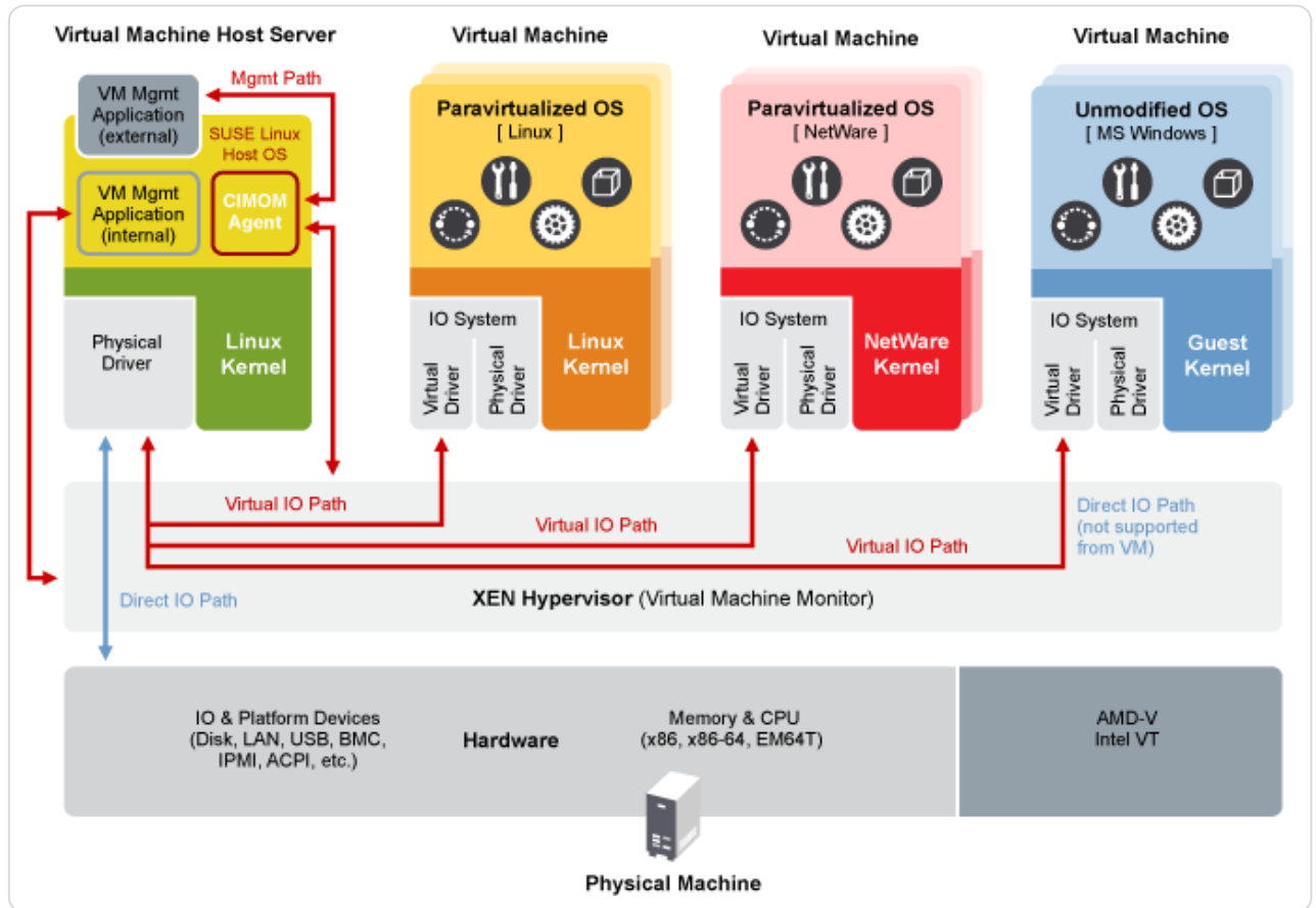
Figure 3.2.1. Xen virtualization architecture
