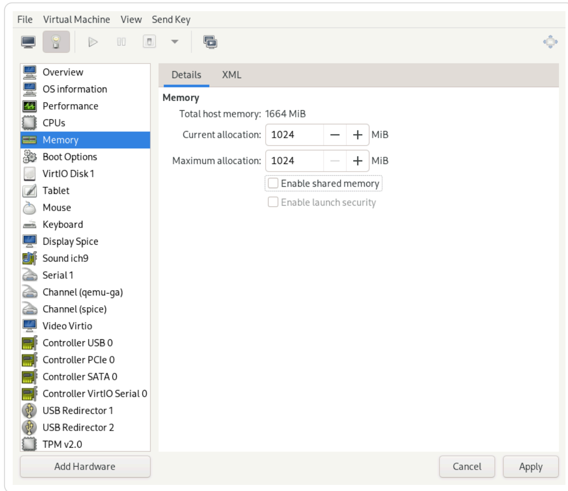
Figure 14.1.4.7. Memory view
