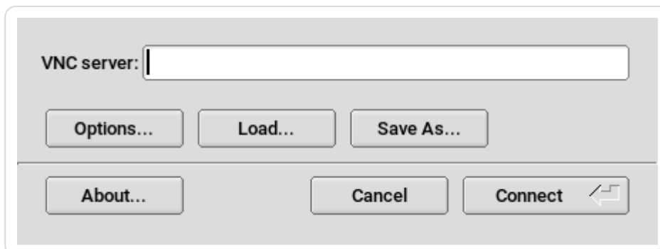
Figure 14.1. vncviewer
