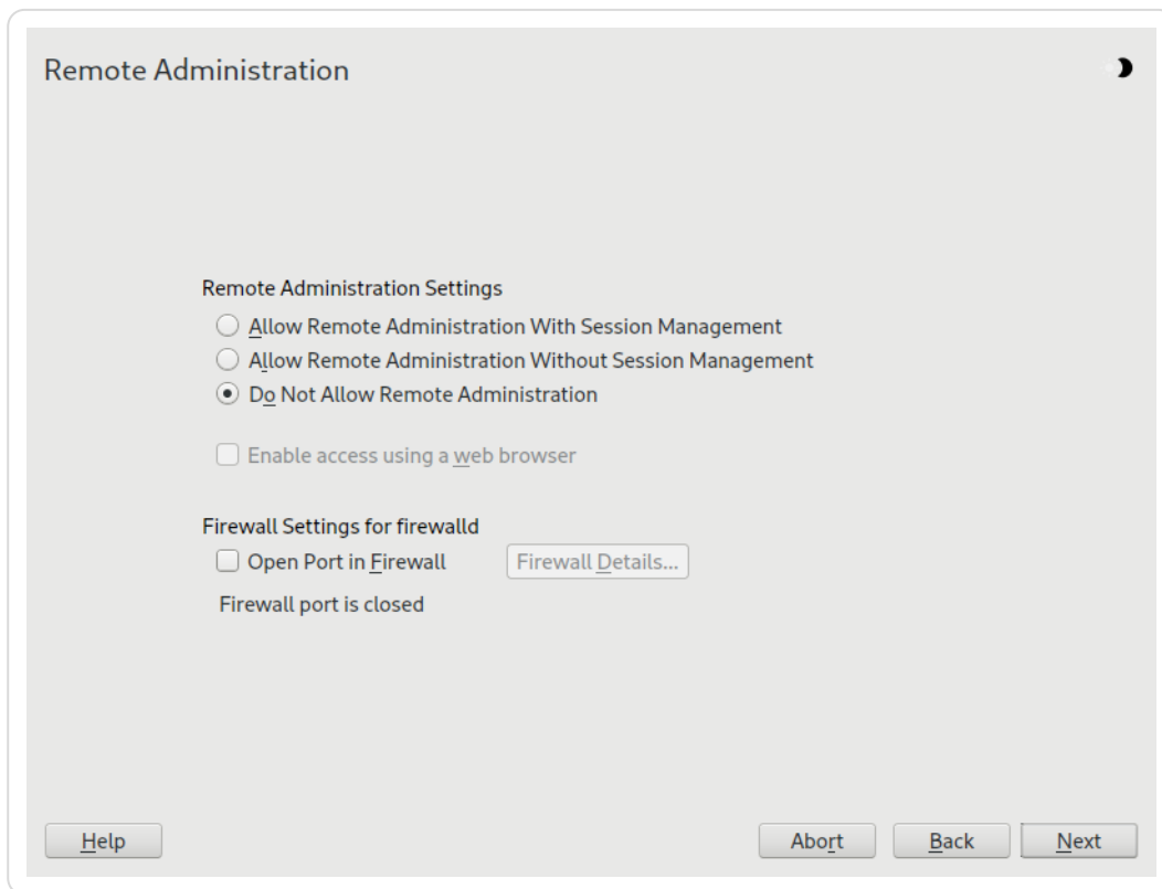
Figure 14.7. Remote administration
