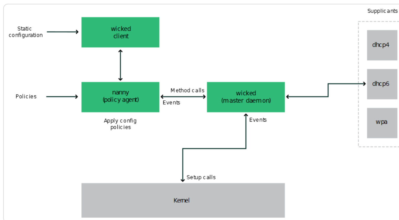
Figure 23.4. wicked architecture
