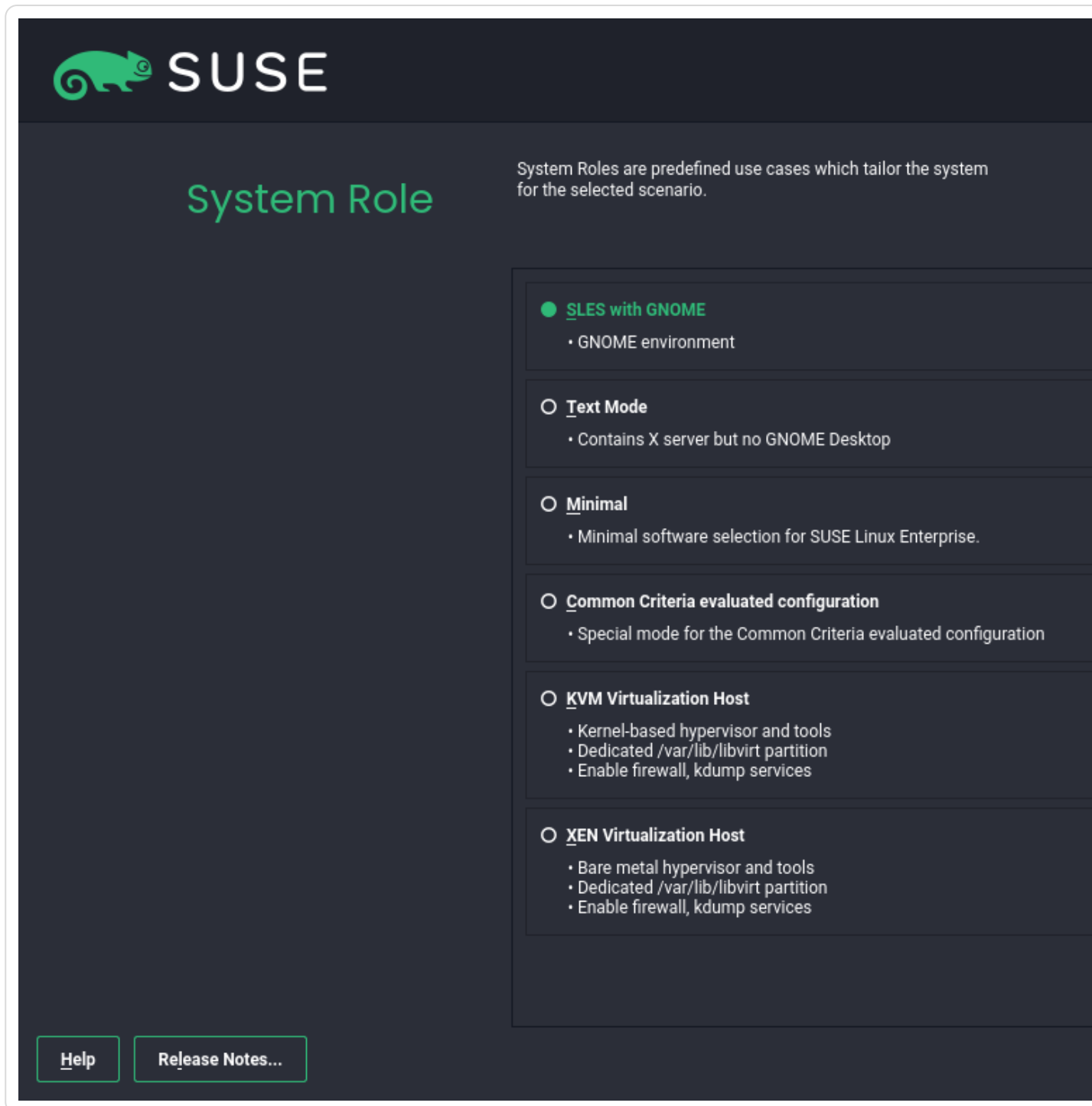
Figure 10.10. System role
