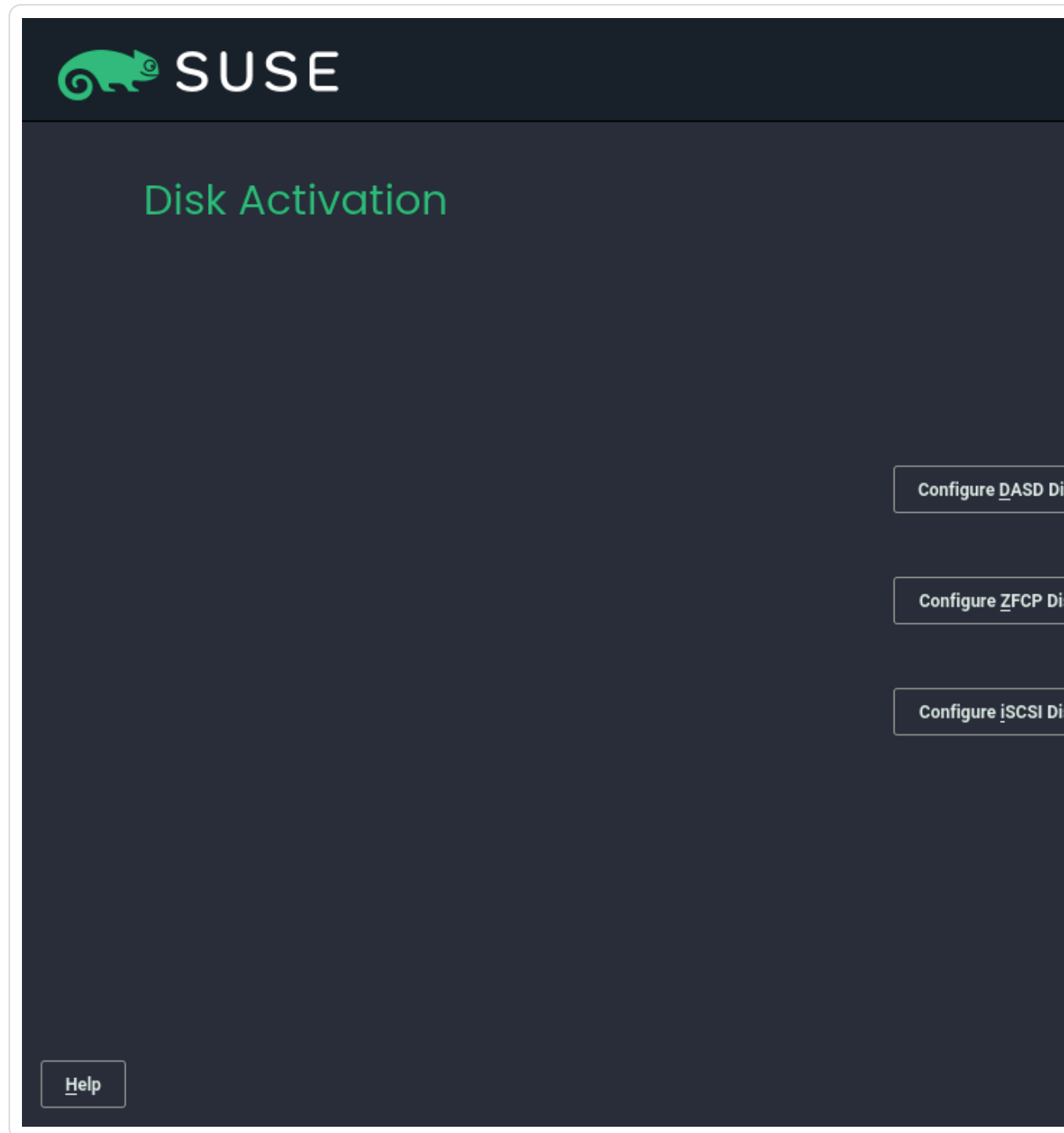
Figure 10.3. Disk activation
