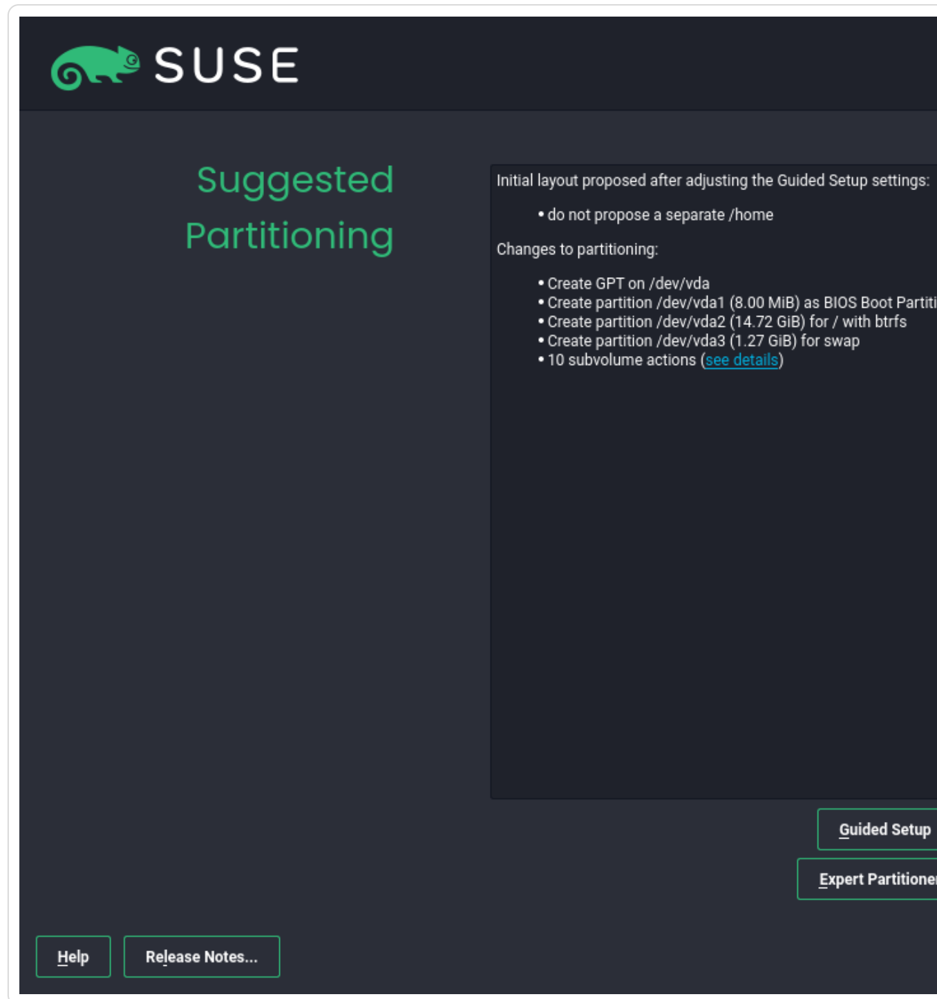
Figure 10.11. Suggested partitioning
