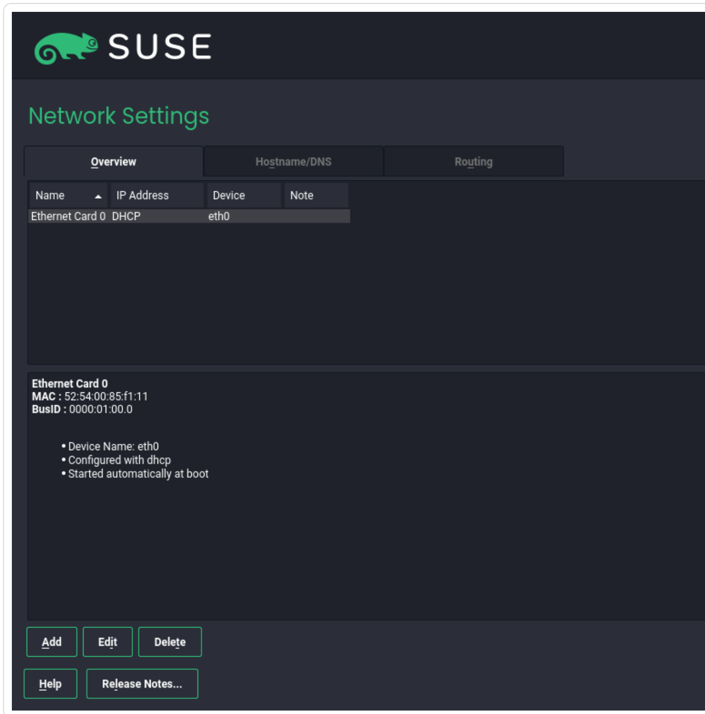
Figure 10.6. Network settings
