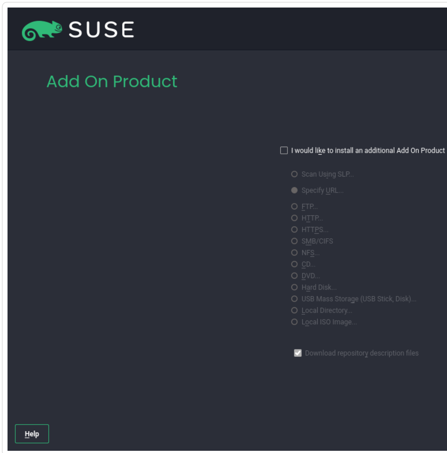
Figure 10.9. Add-on product
