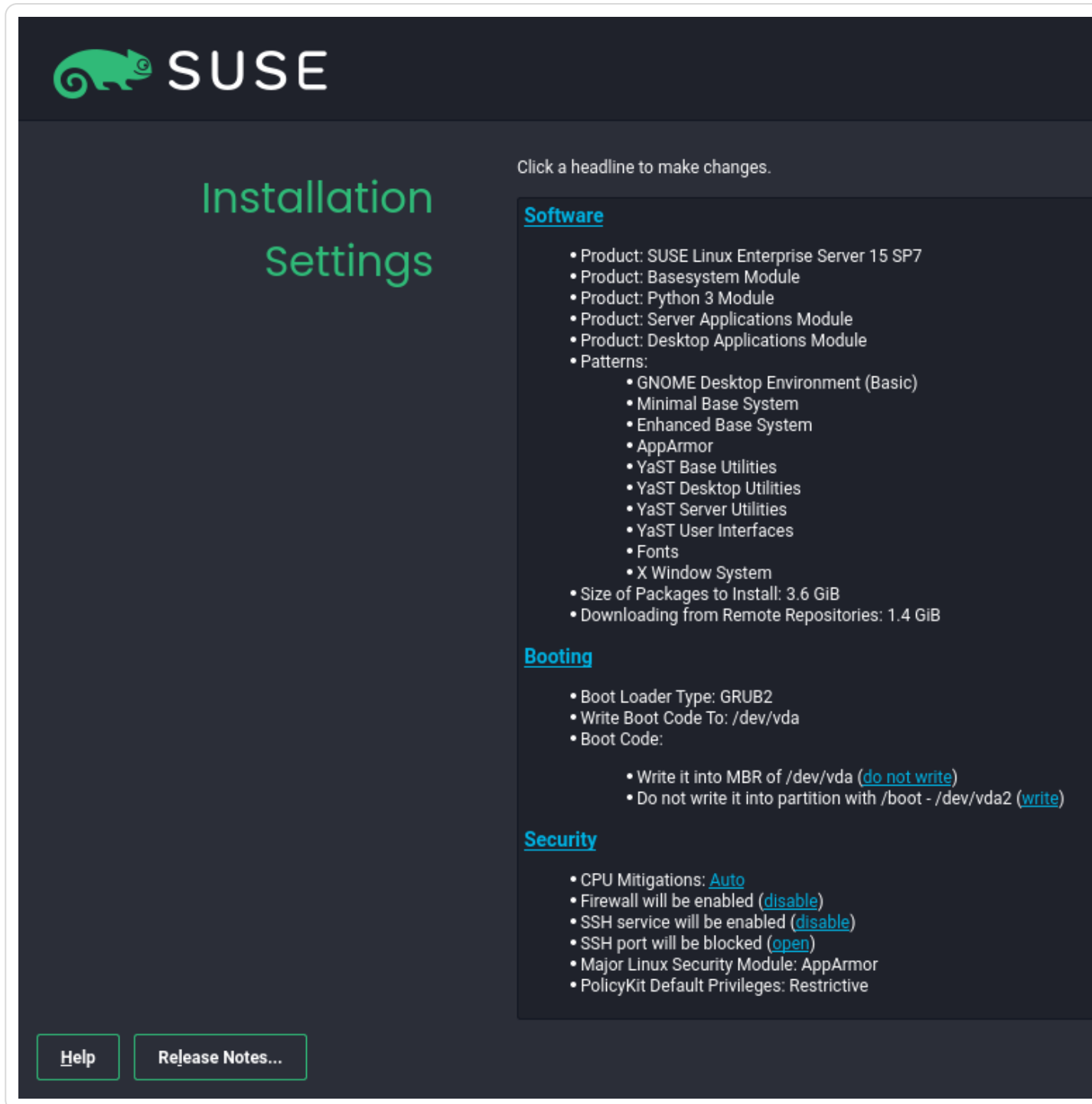
Figure 10.15. Installation settings
