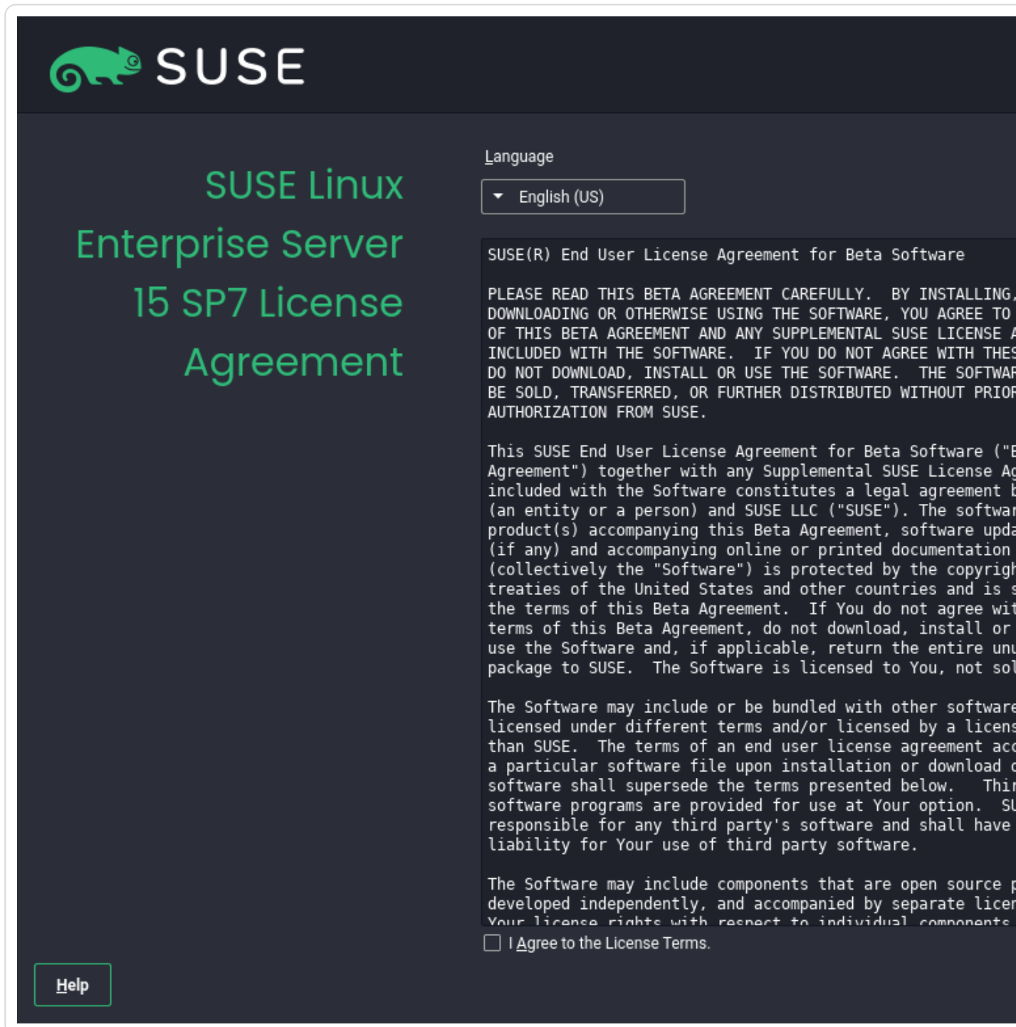
Figure 10.2. License agreement
