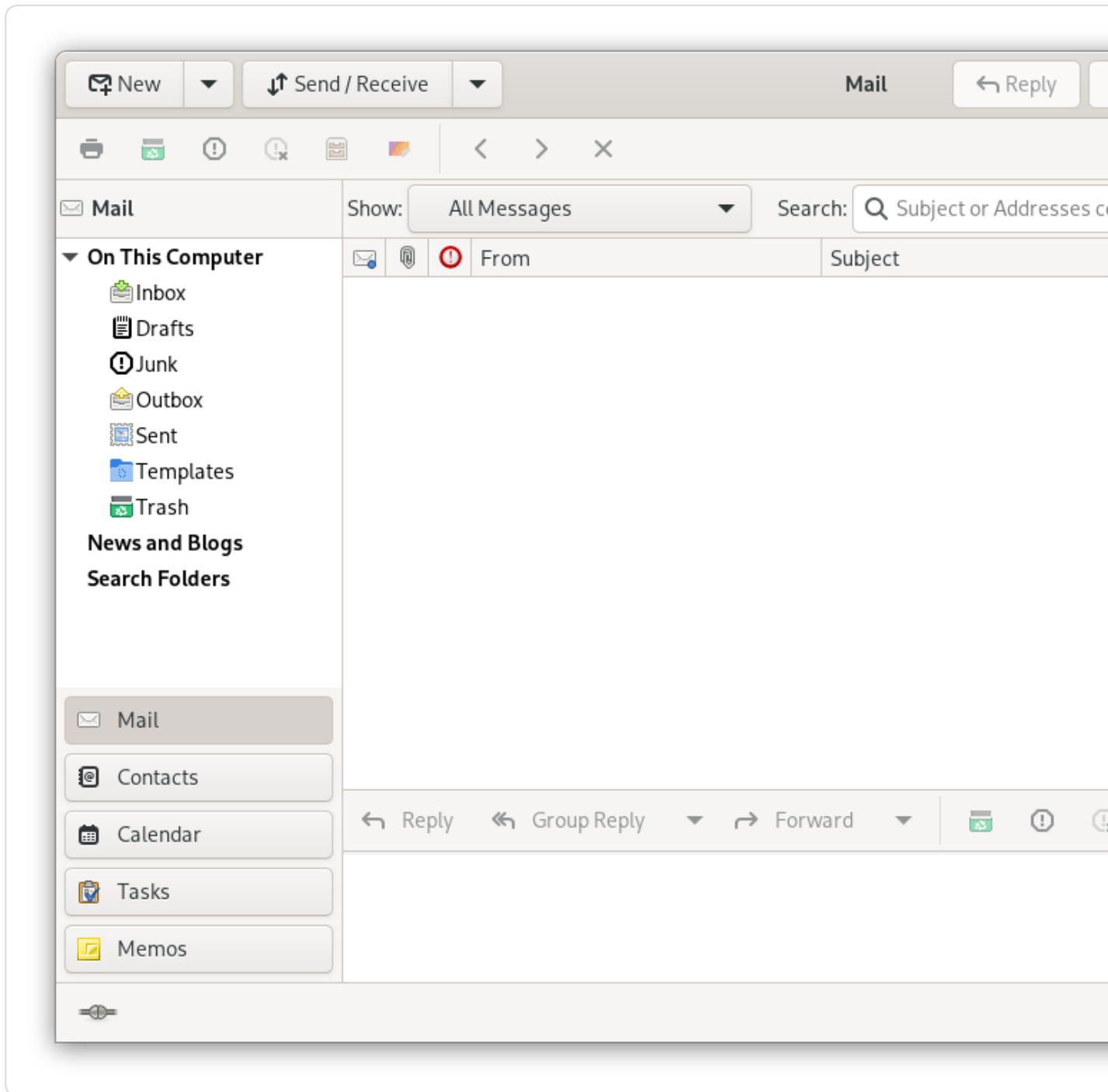
Figure 14.1. Evolution window
