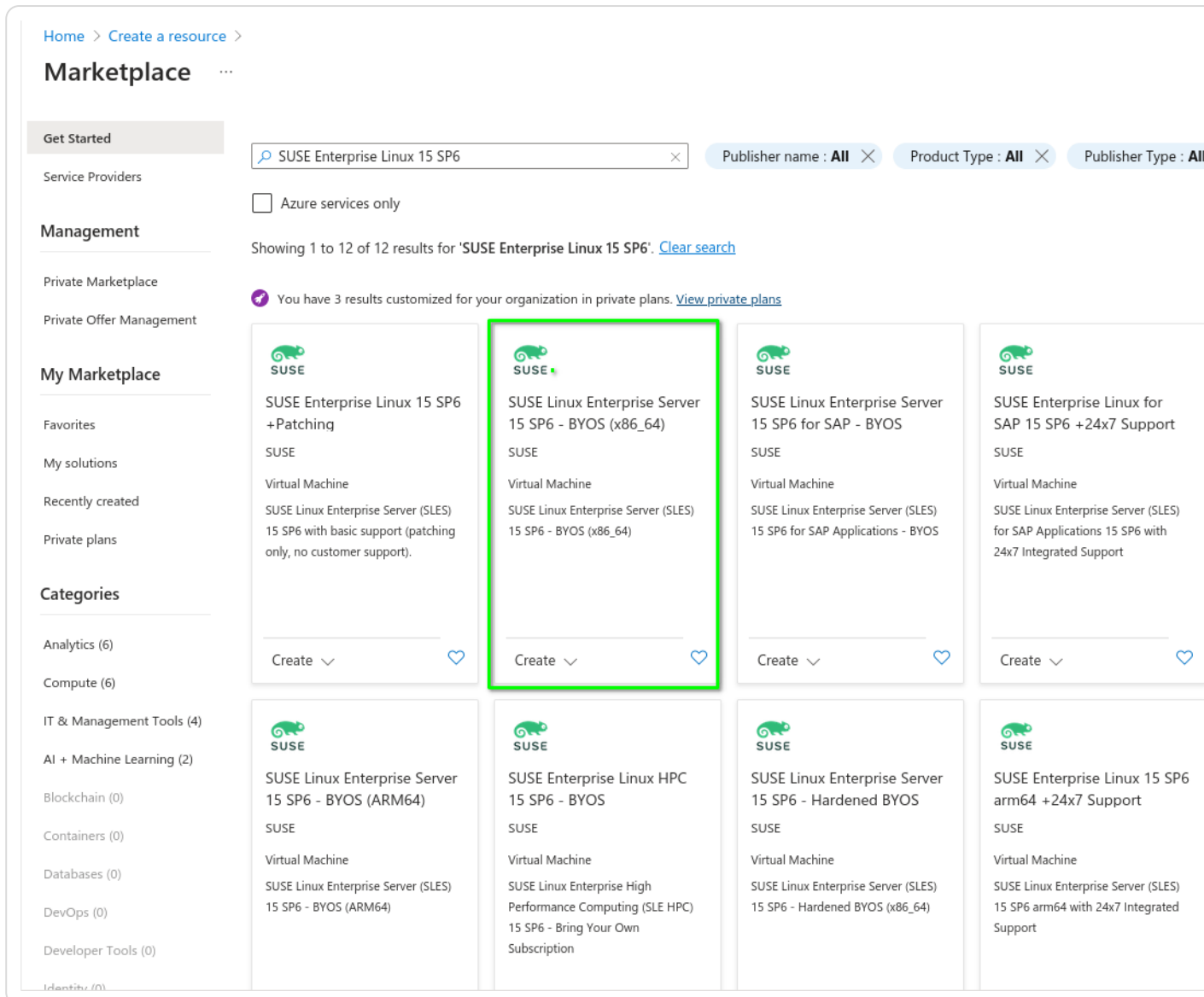
Figure 9.4. Microsoft Azure
