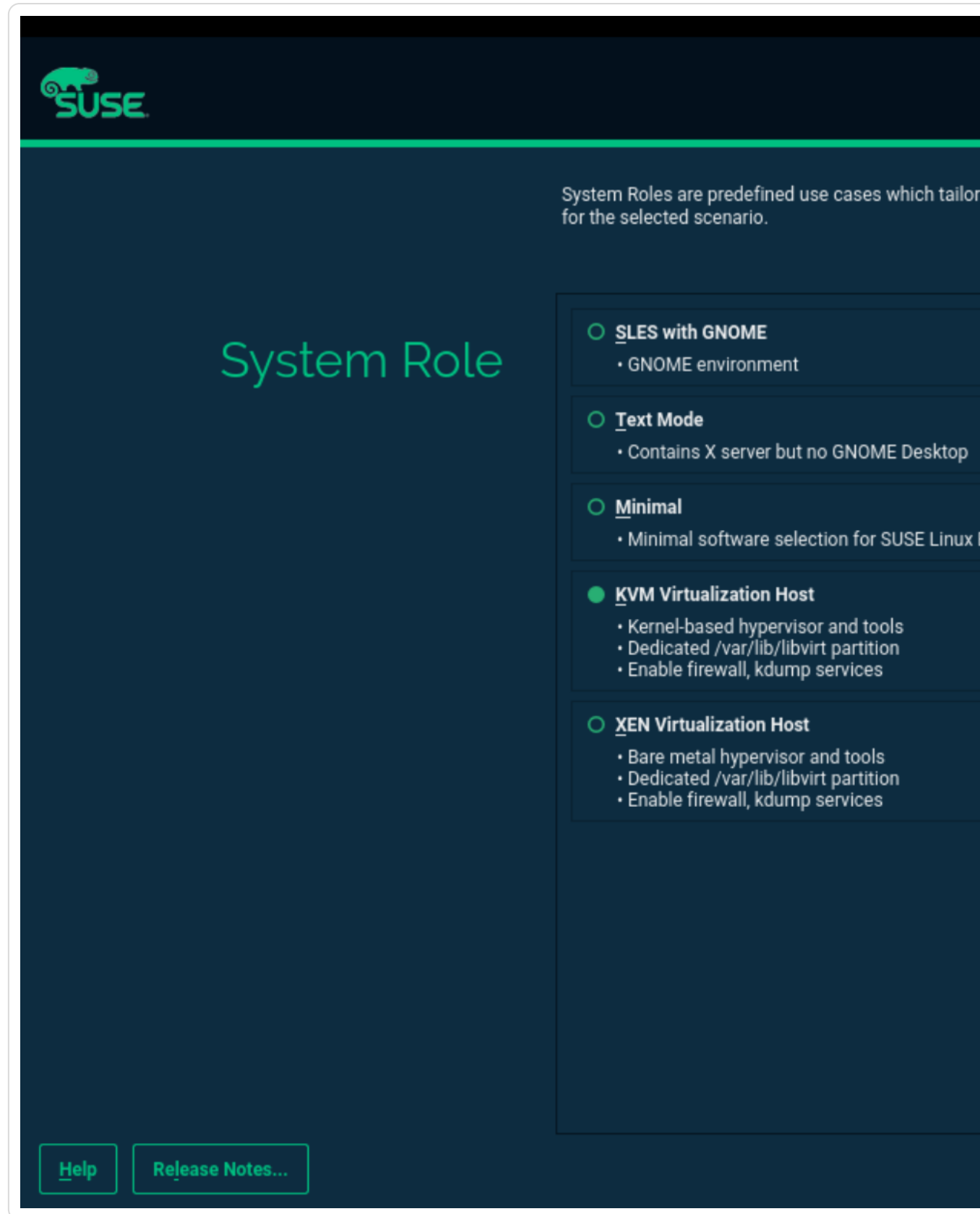
Figure 6.1. System Role screen
