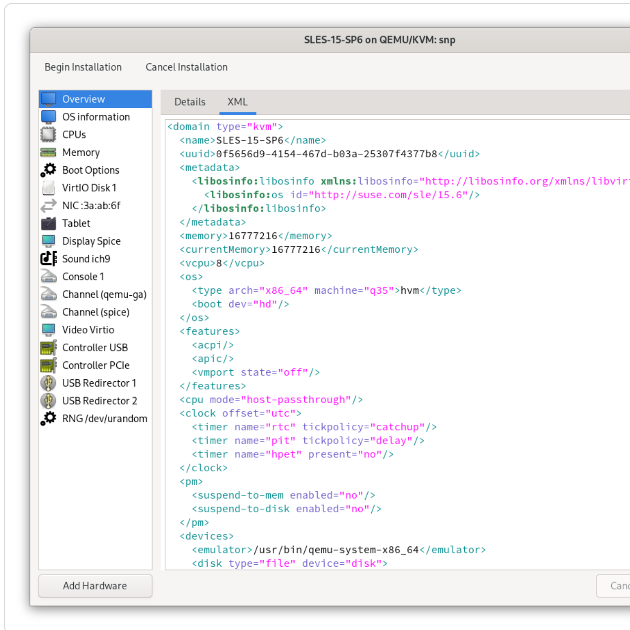
Figure 16.2. XML view of virtual machine configuration
