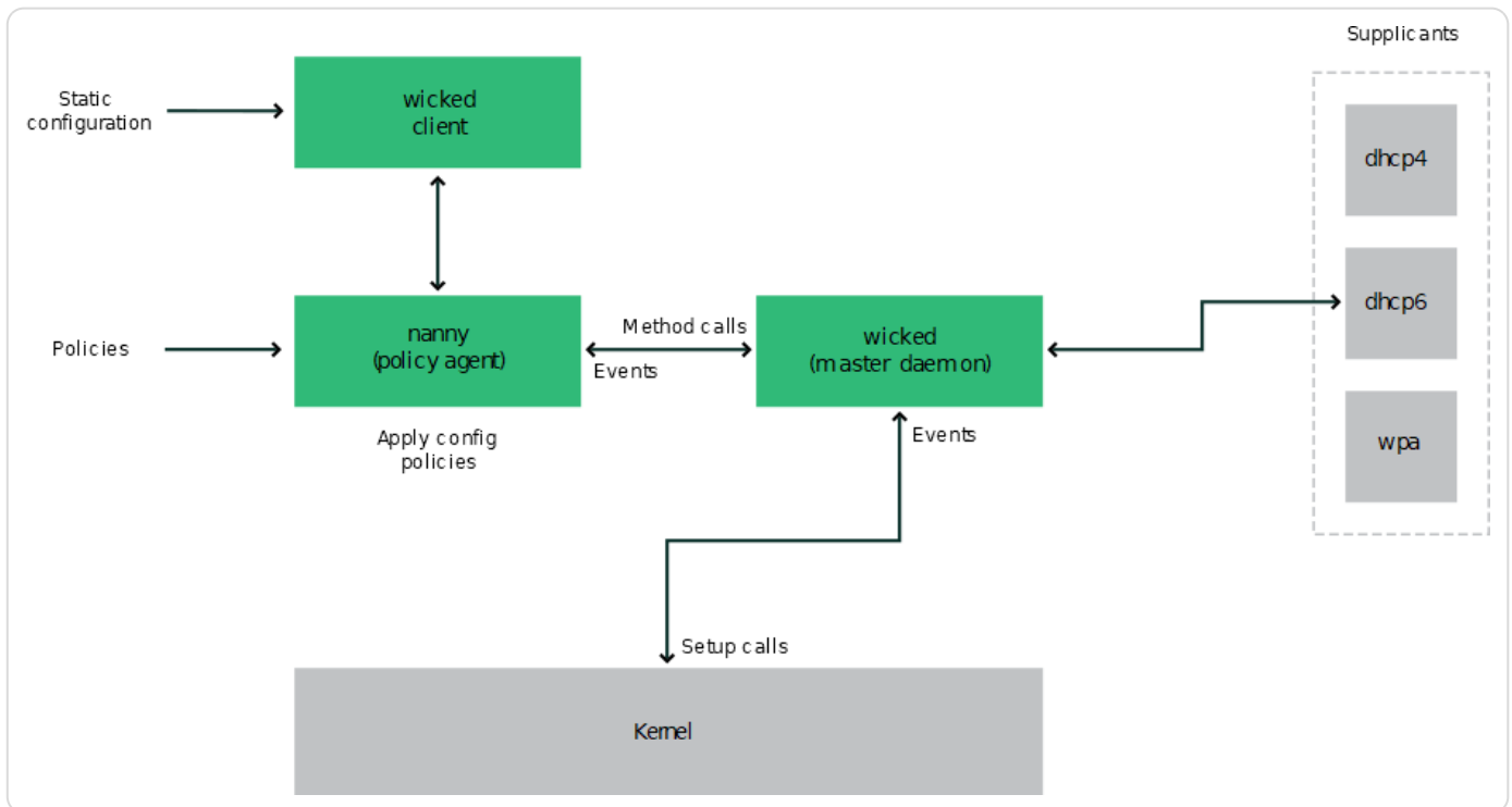
Figure 23.4. wicked architecture
