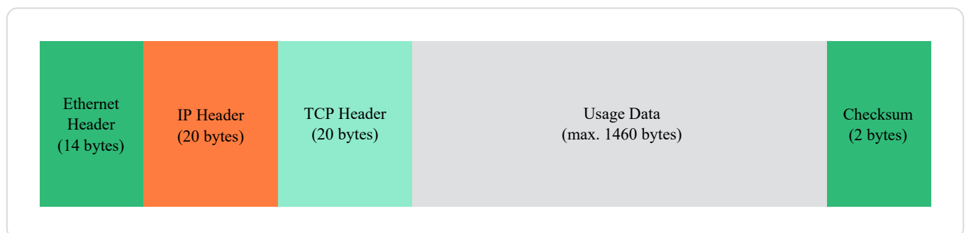
Figure 23.2. TCP/IP Ethernet packet
