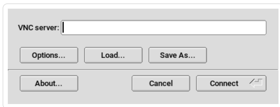
Figure 14.1. vncviewer
