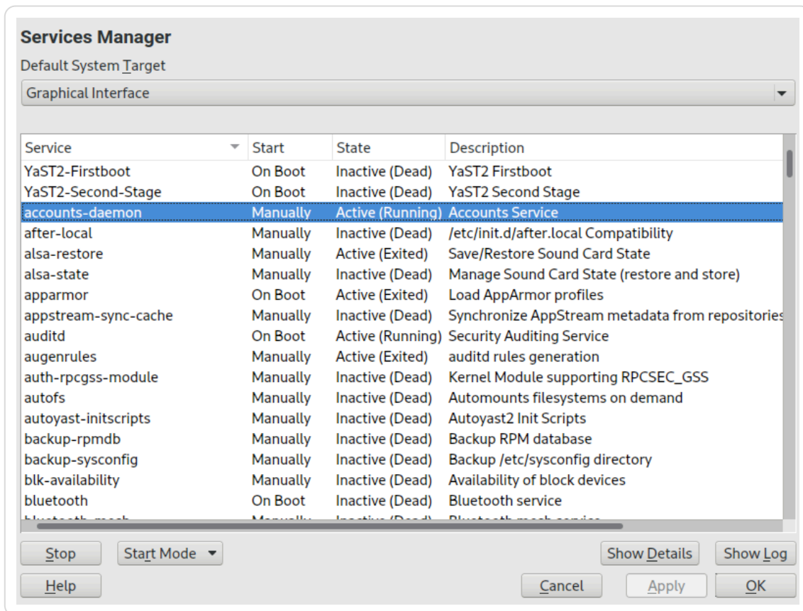
Figure 19.1. Services Manager
