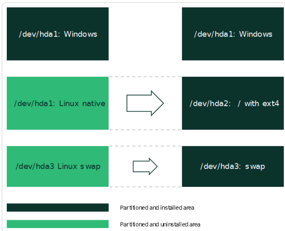
Figure 4.1. Keeping partitions
