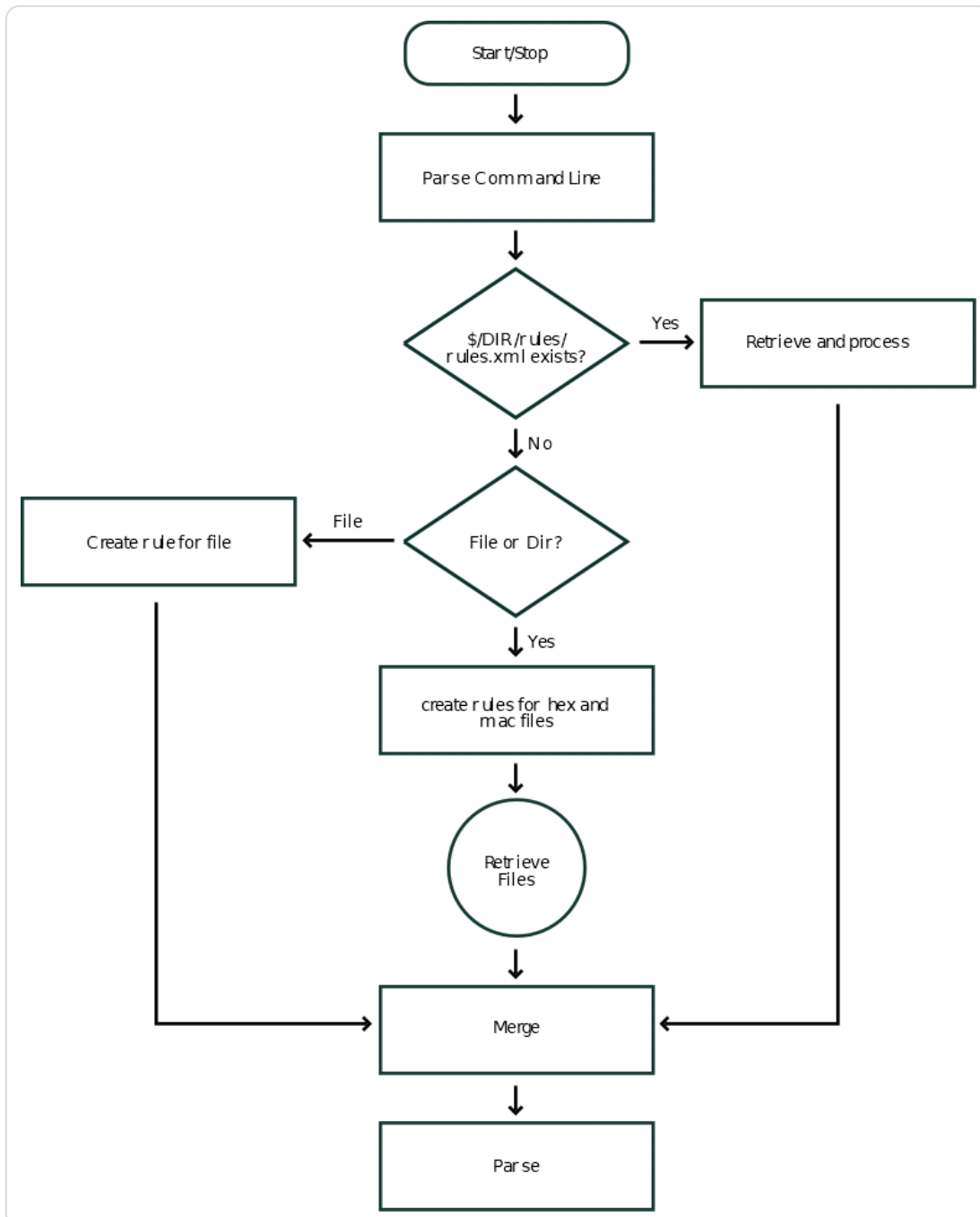
Figure A.1. Rules retrieval process
