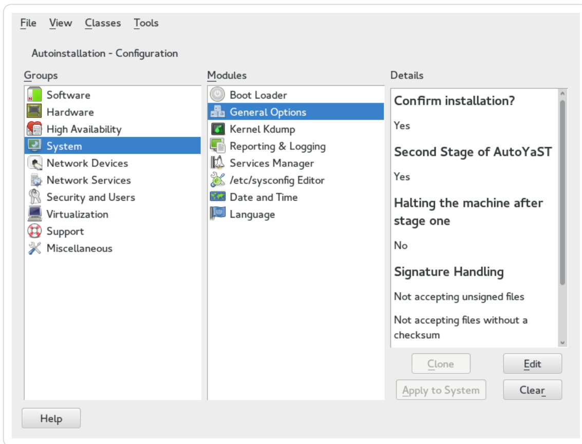
Figure 3.1. Configuration system
