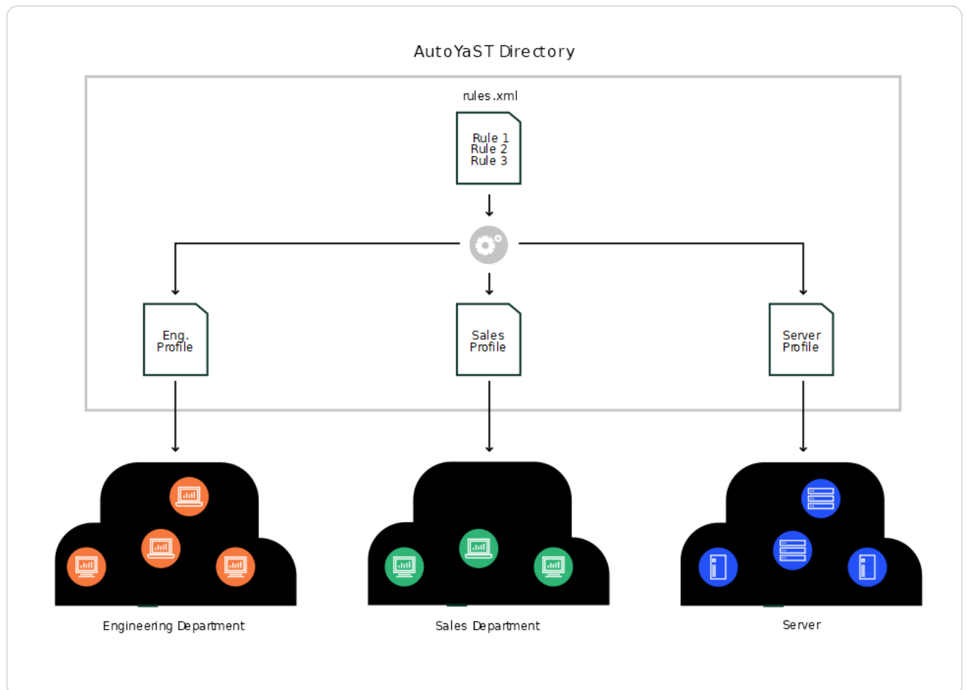
Figure 6.1. Rules
