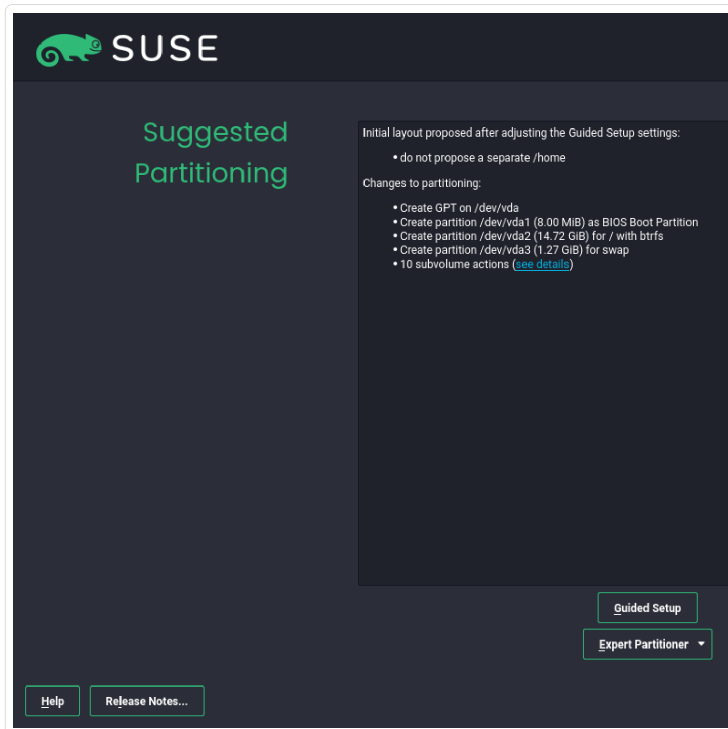
Figure 10.11. Suggested partitioning
