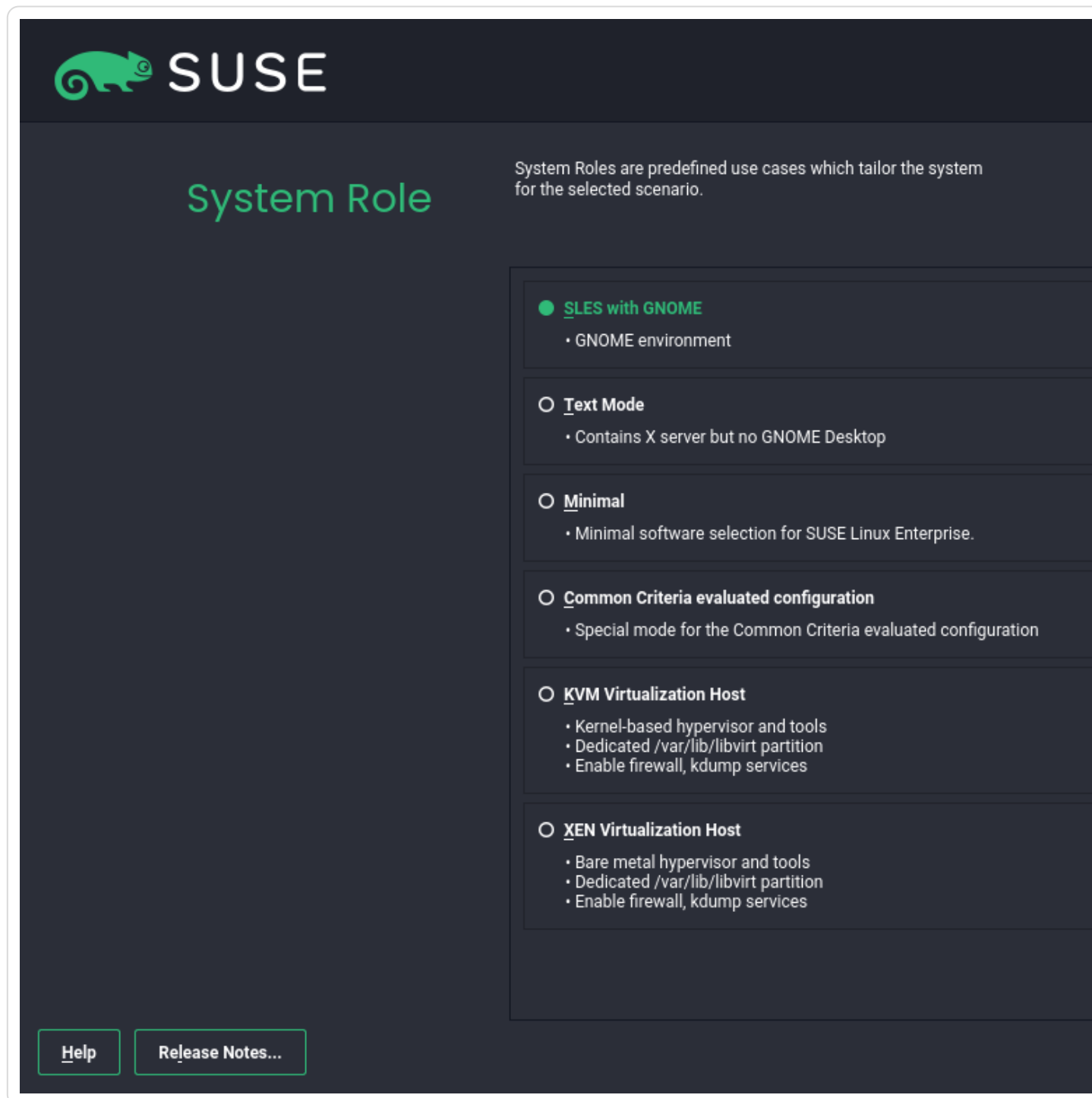
Figure 10.10. System role
