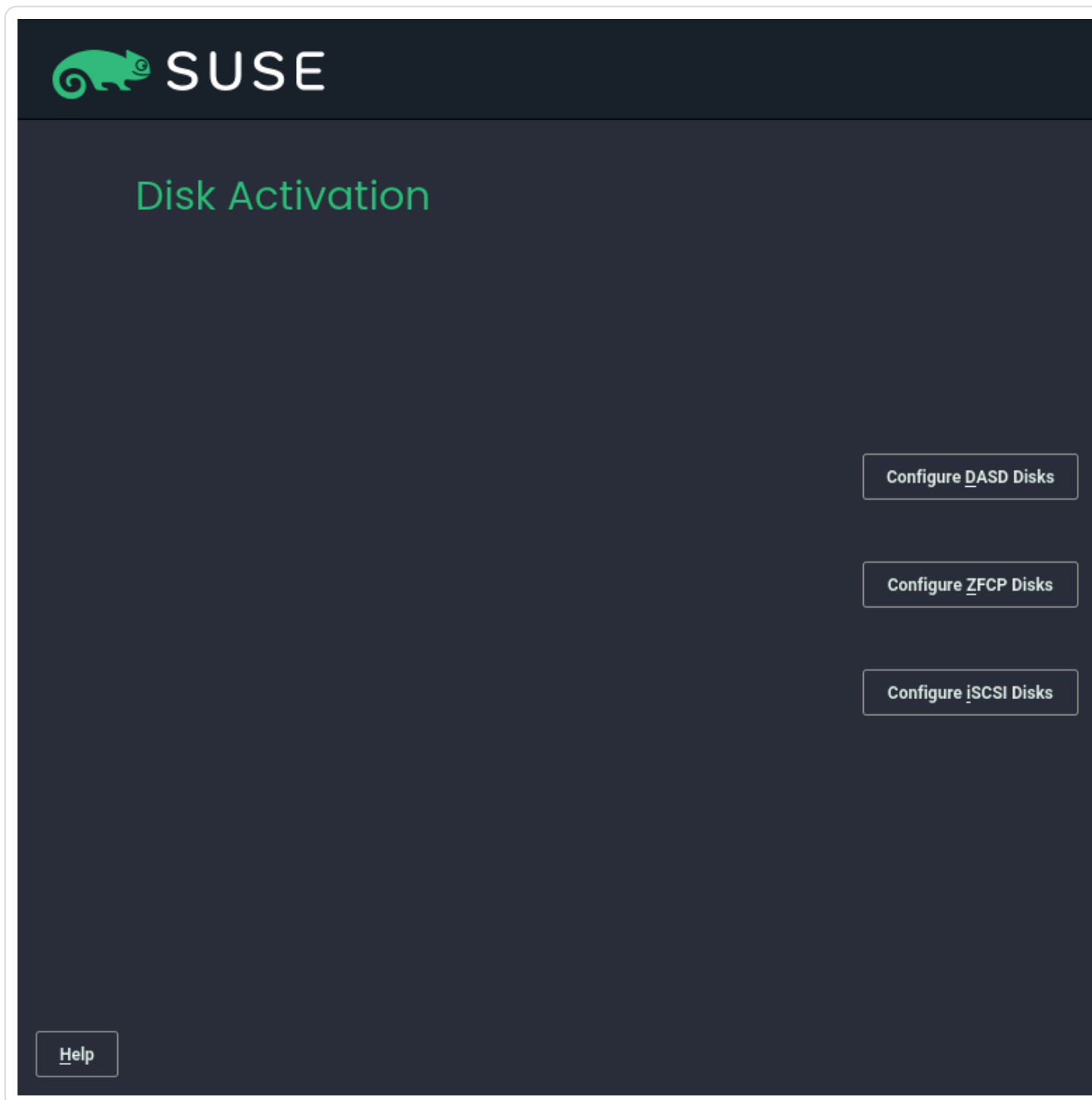
Figure 10.3. Disk activation
