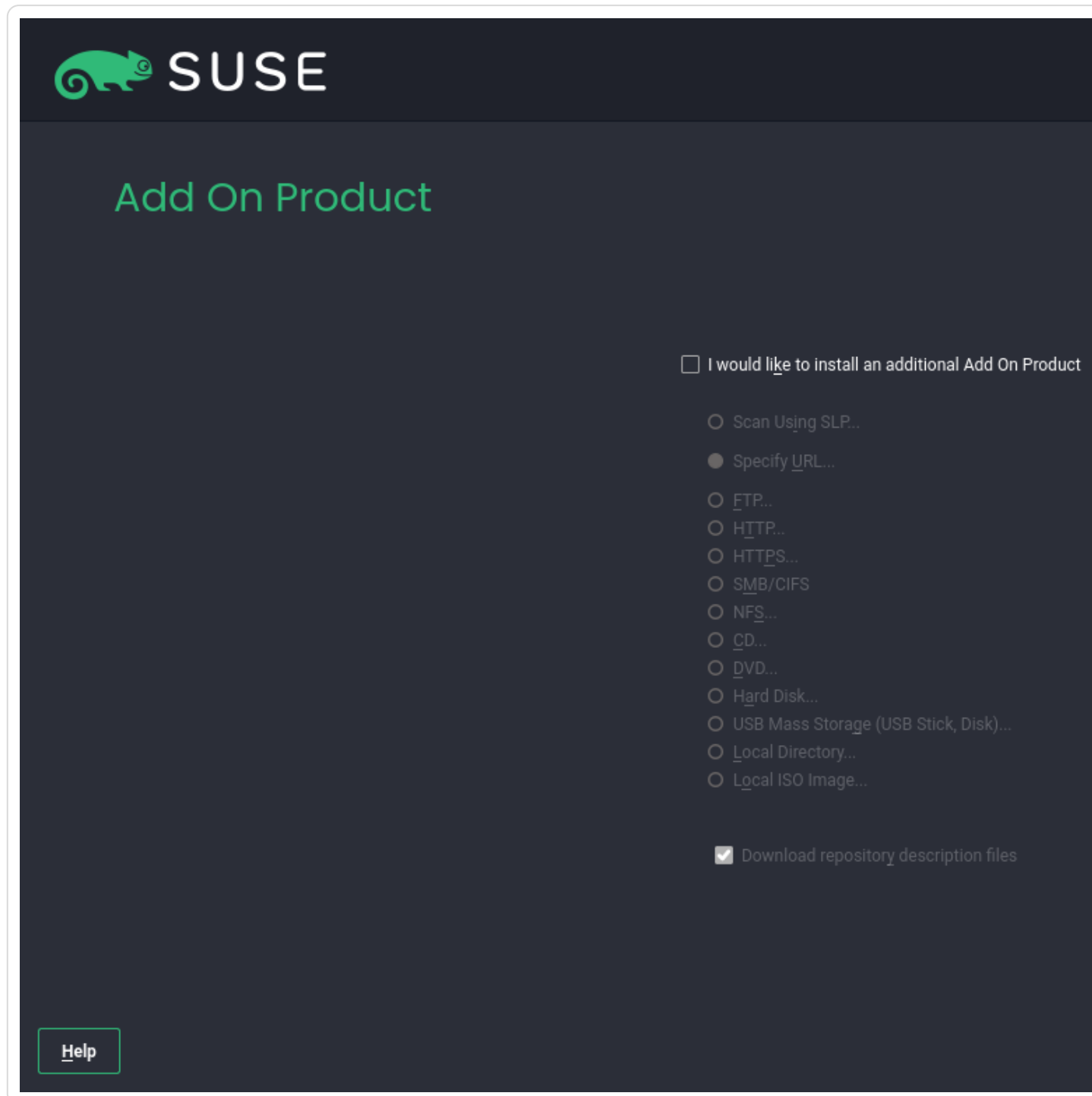
Figure 10.9. Add-on product
