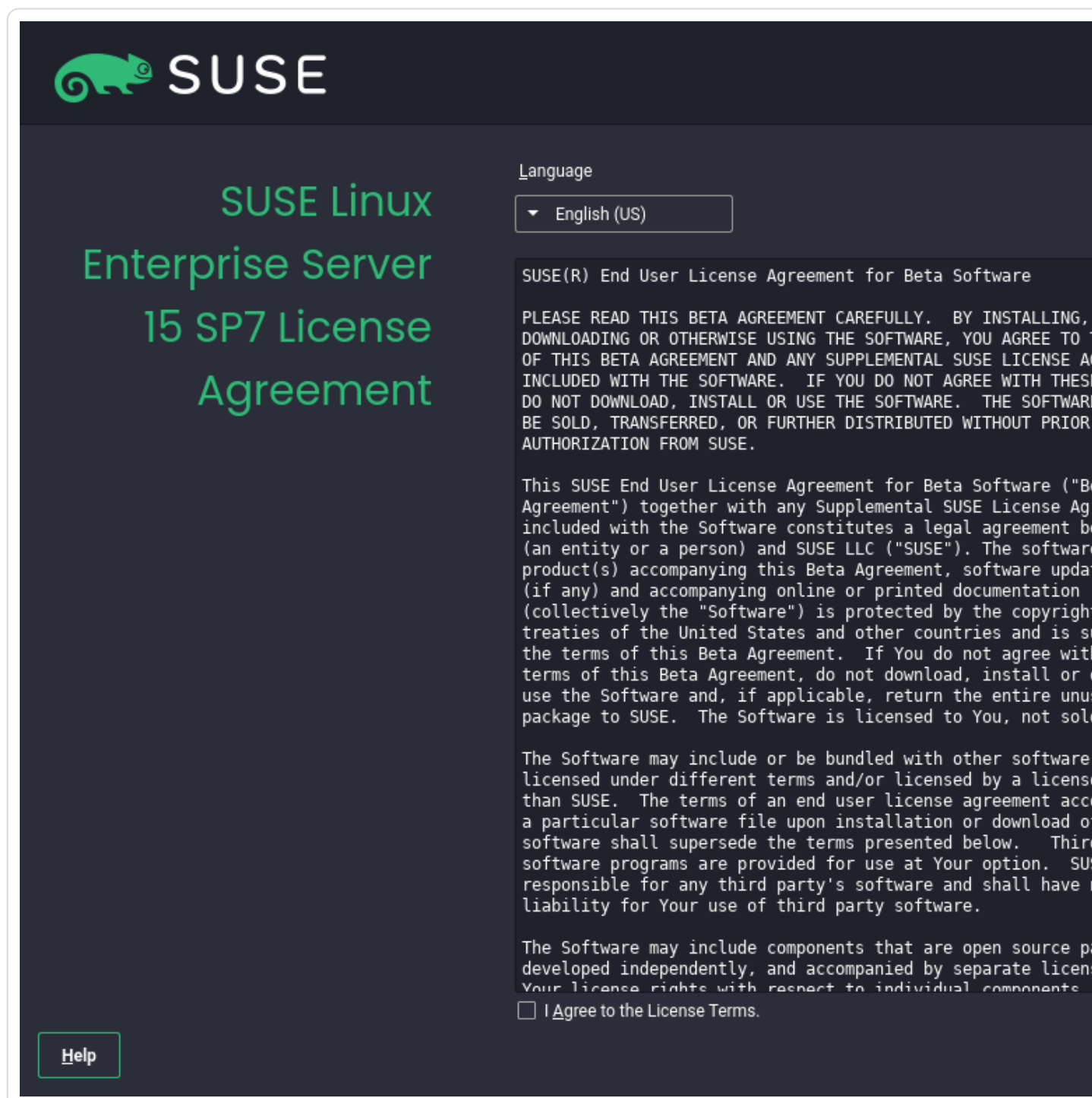
Figure 10.2. License agreement
