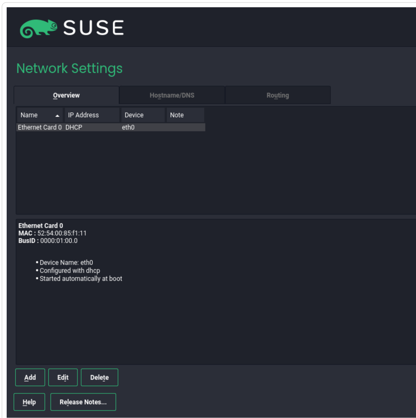
Figure 10.6. Network settings
