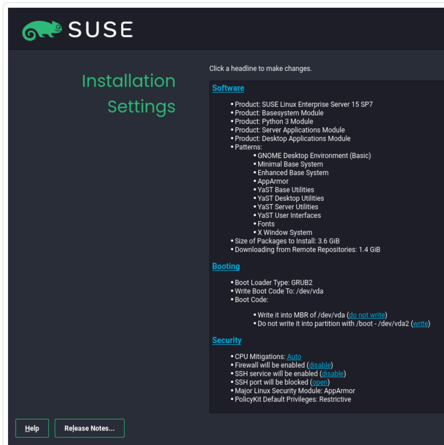
Figure 10.15. Installation settings
