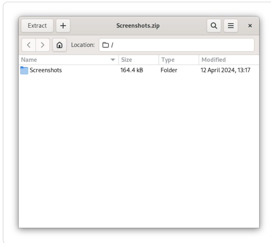
Figure 2.2. Archive manager
