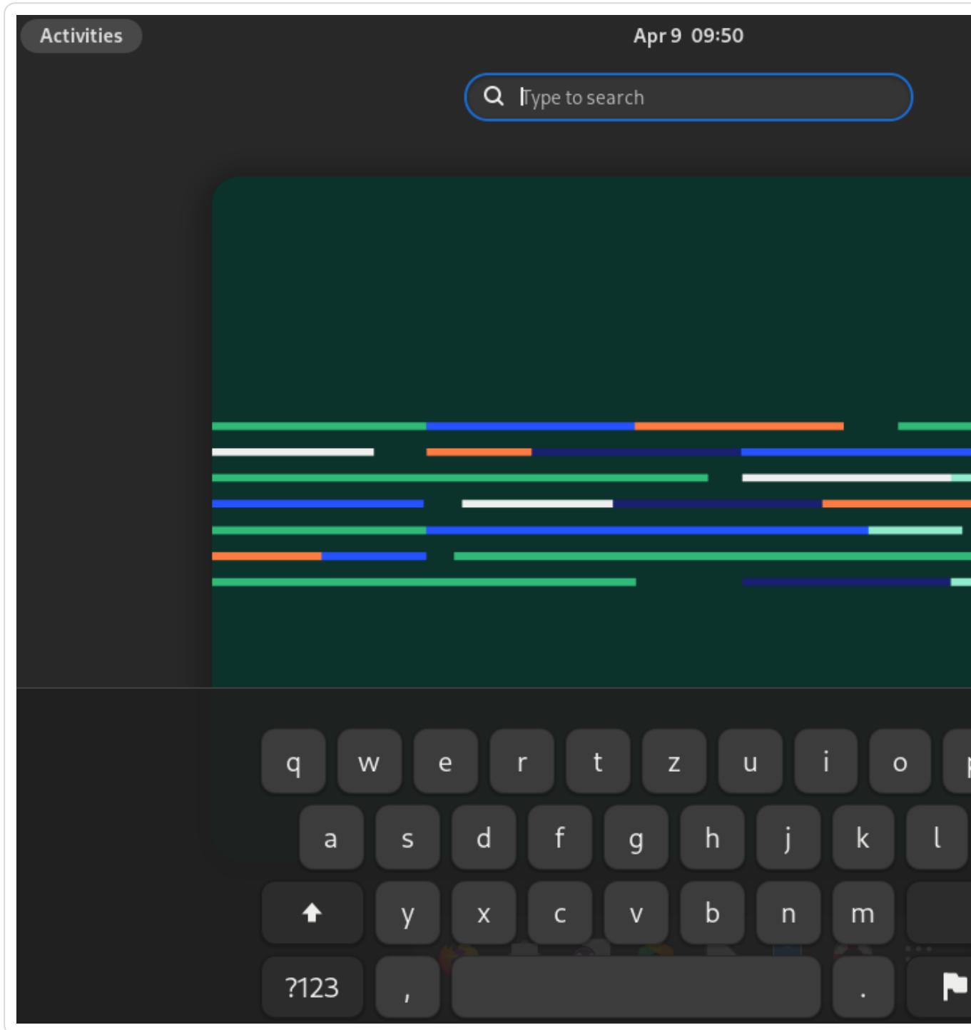
Figure 4.1. On-screen keyboard
