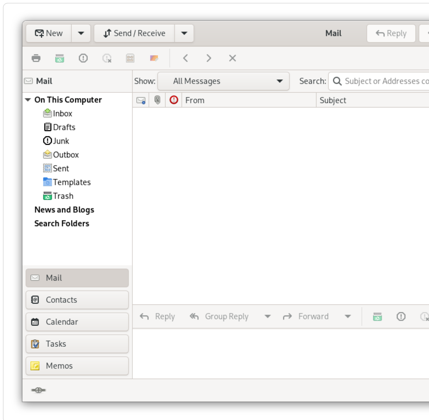
Figure 14.1. Evolution window
