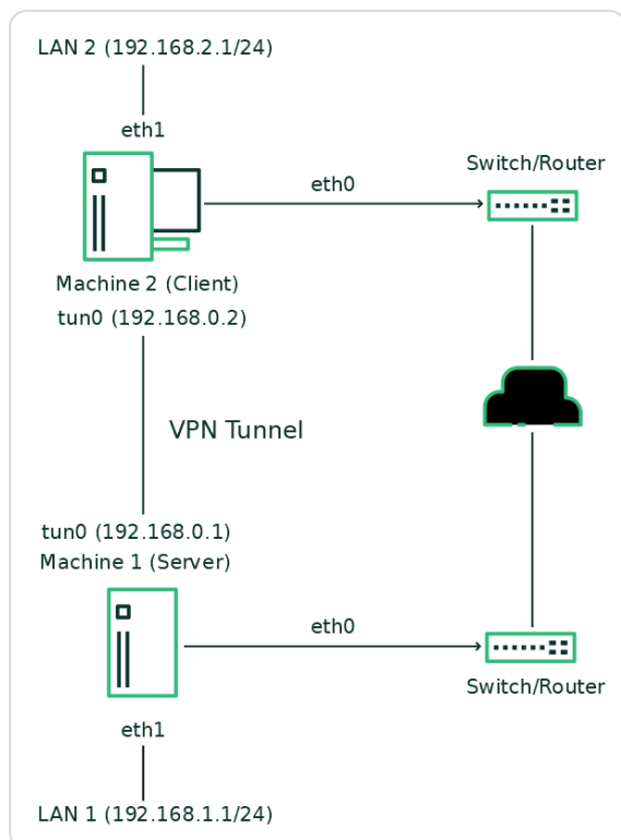
Figure 24.1. Routed VPN
