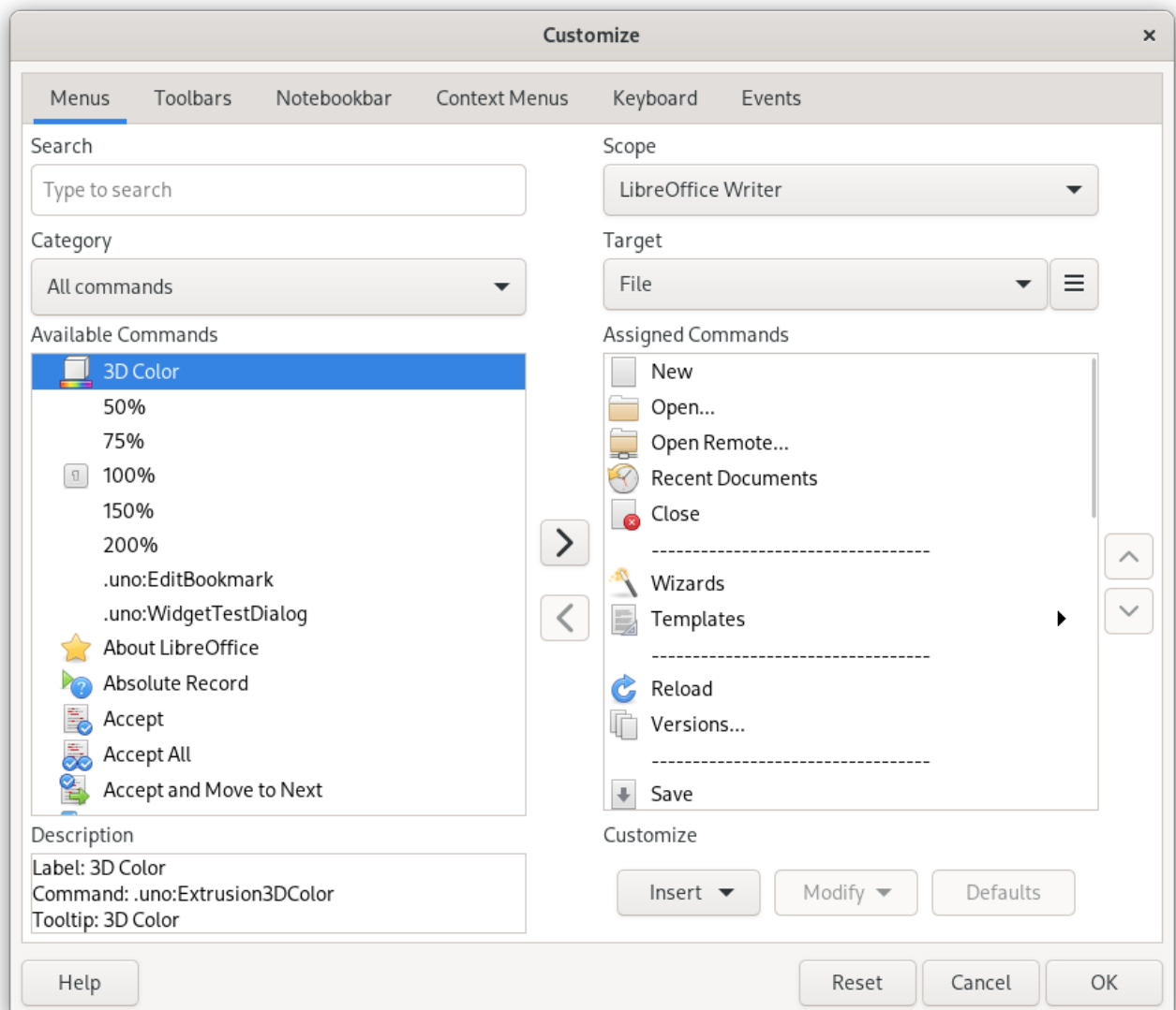
Figure 9.1. Customization dialog in Writer
