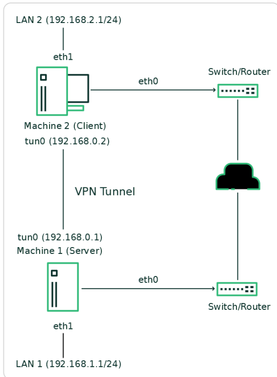
Figure 24.1. Routed VPN
