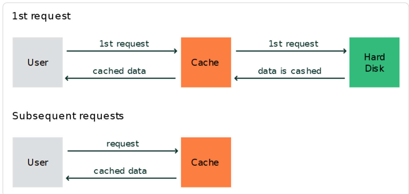
Figure 19.1. Caching mechanism
