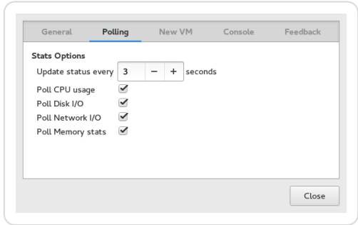
Figure 14.5. Statistics charts
