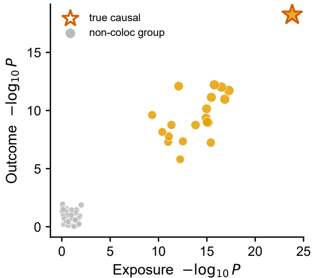
One causal variant coloc PP.H4=1.00
