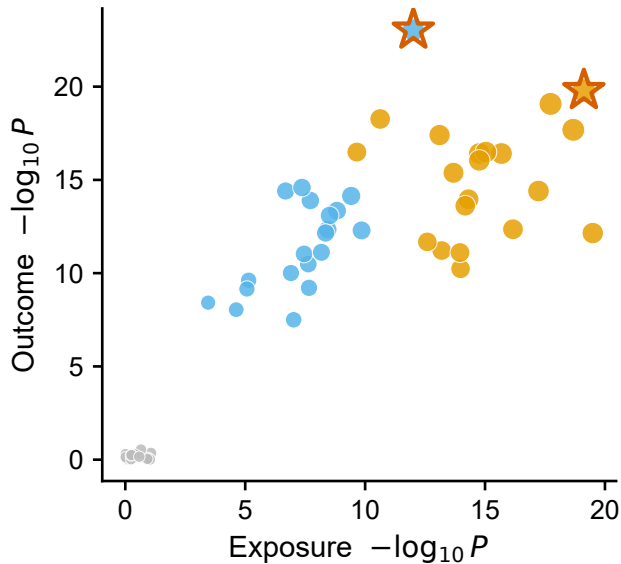
Two causal variants coloc PP.H4=0.15
