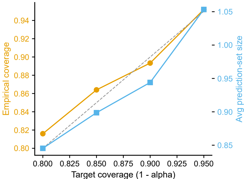
Coverage vs efficiency trade-off
