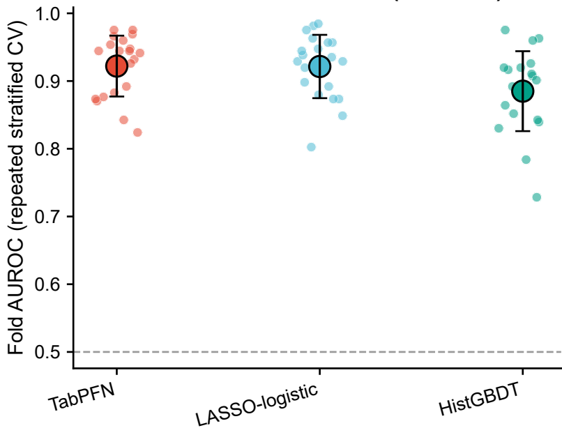
Cross-validated AUROC (5×4 folds)
