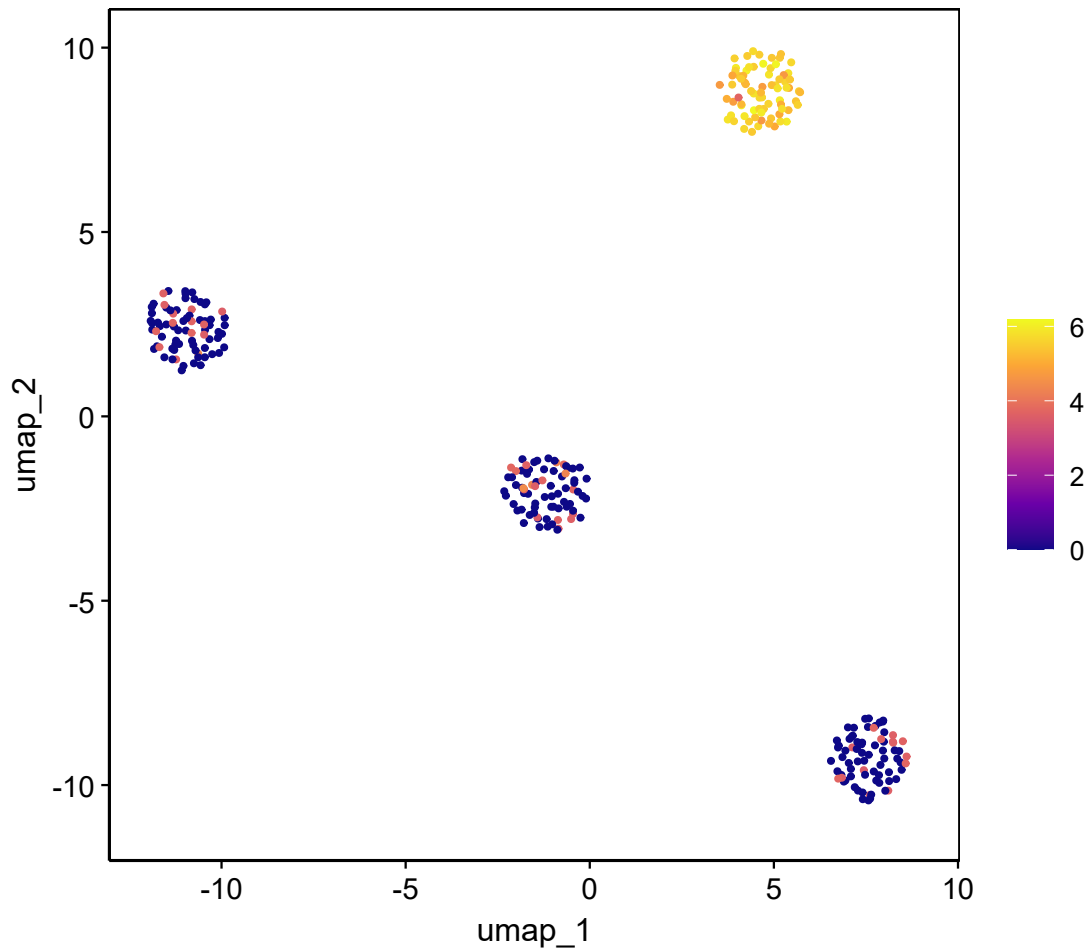
Bcell-m16 (UMAP)
