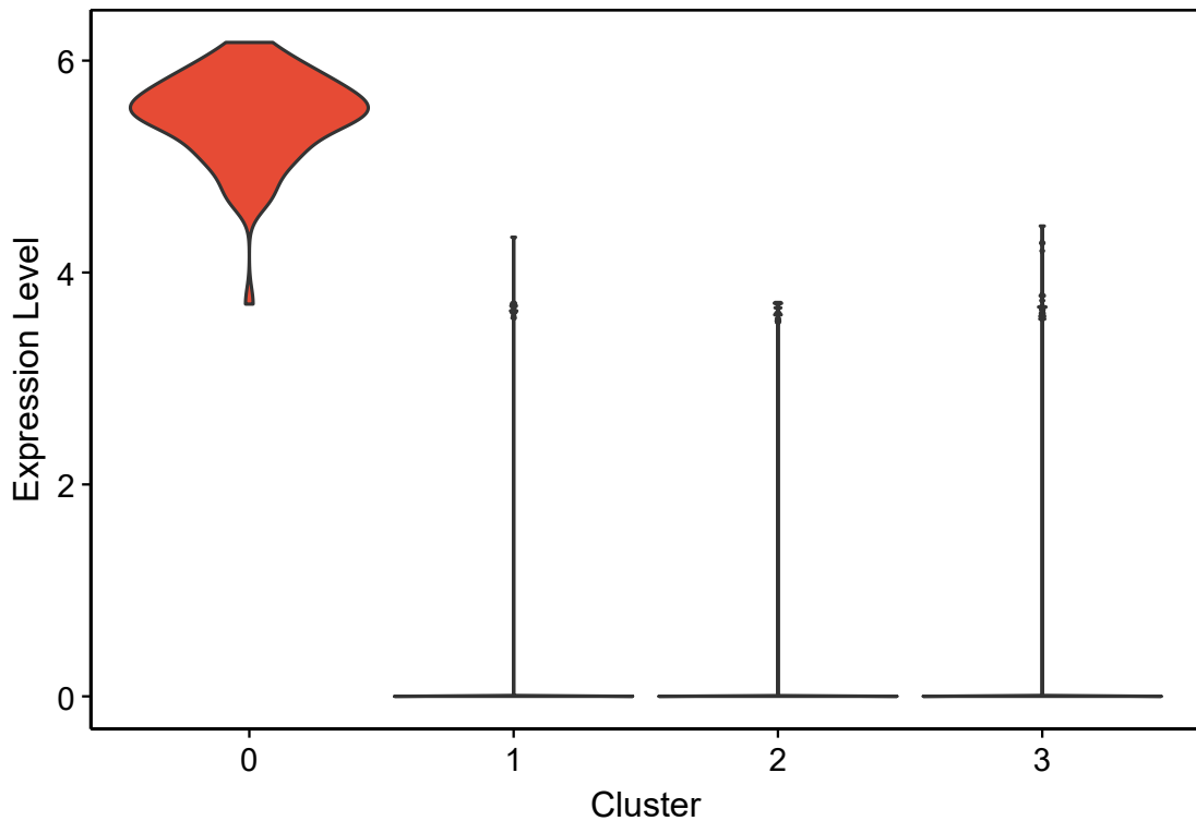
Bcell-m16 by cluster
