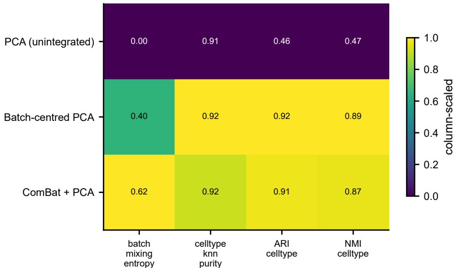
Integration metrics (cell = raw value, colour = column-scaled)
