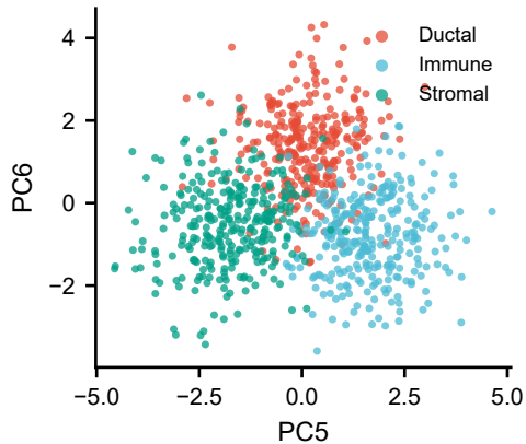
PCA embedding (most cell-type-informative PCs)
