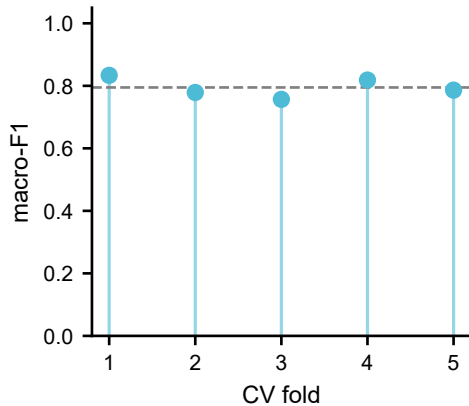
Cell-type prediction (PCA + kNN floor)
