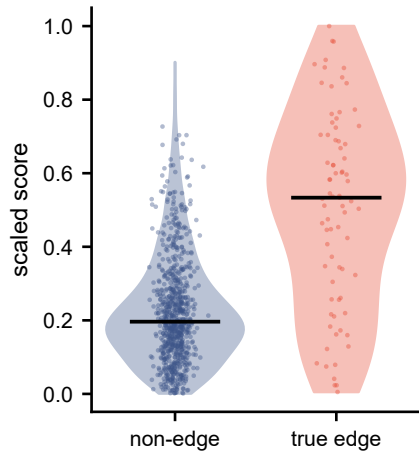
Score separation
